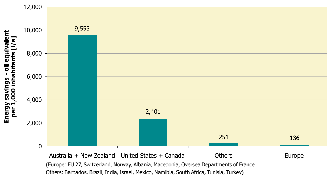
Figure 22: Annual energy savings by economic region at the end of 2005 per 1,000 inhabitants in oil equivalent – unglazed collectors
