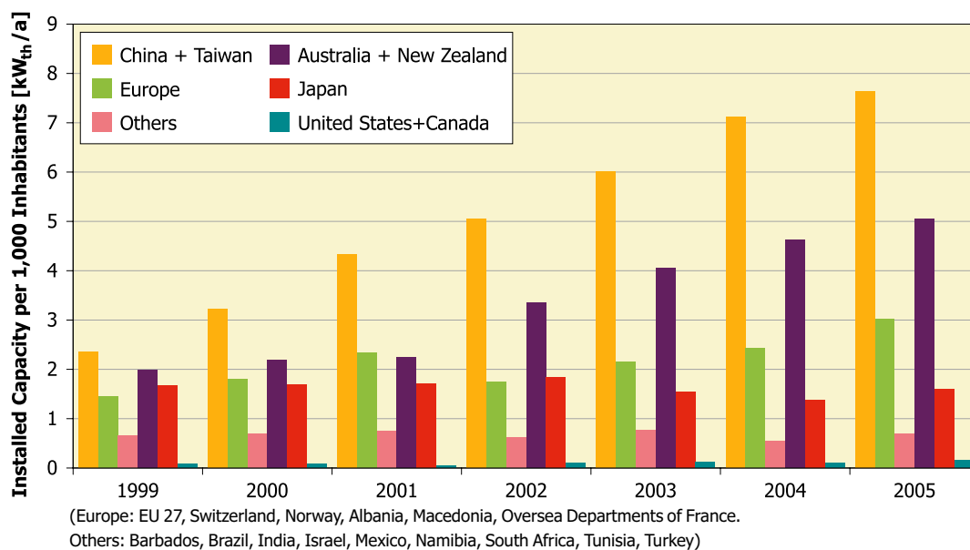
Figure 13b: Annual installed capacity of flat plate and evacuated tube collectors in \text{kW}_{\text{th}} per 1,000 inhabitants
