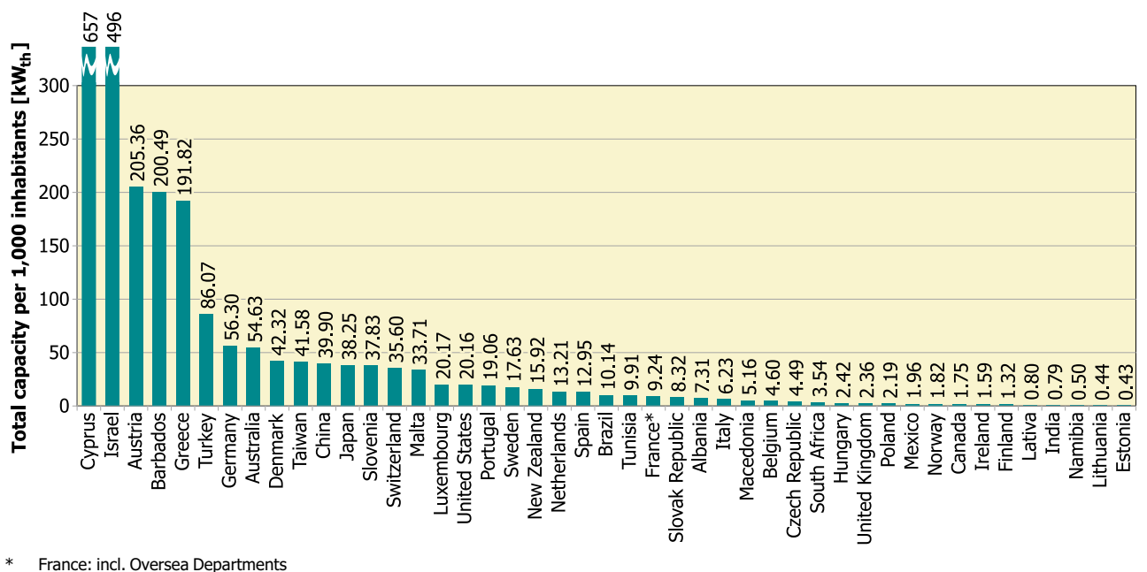
Figure 6: Total capacity of glazed flat plate and evacuated tube collectors in operation at the end of 2005 in kW th per 1,000 inhabitants
