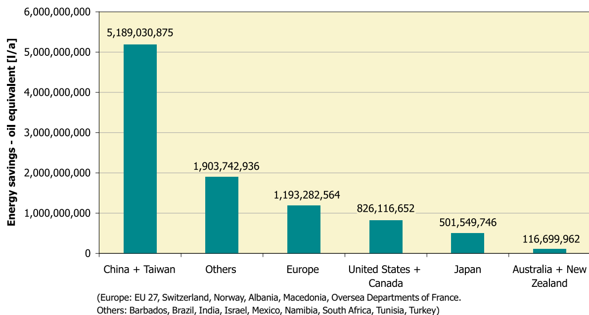
Figure 19: Annual energy savings in oil equivalent – glazed flat plate and evacuated tube collectors by economic region at the end of 2005
