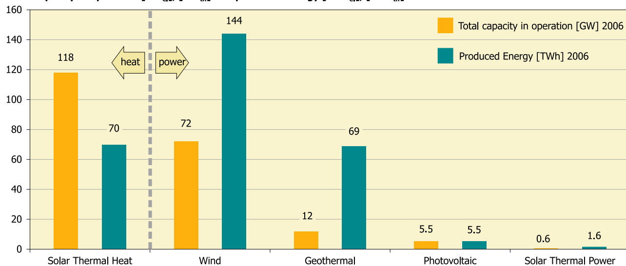
Figure 2: Total capacity in operation [ \text{GW}_{\text{el}} ], [ \text{GW}_{\text{th}} ] 2006 and annually energy generated [ \text{TWh}_{\text{el}} ], [ \text{TWh}_{\text{th}} ].
