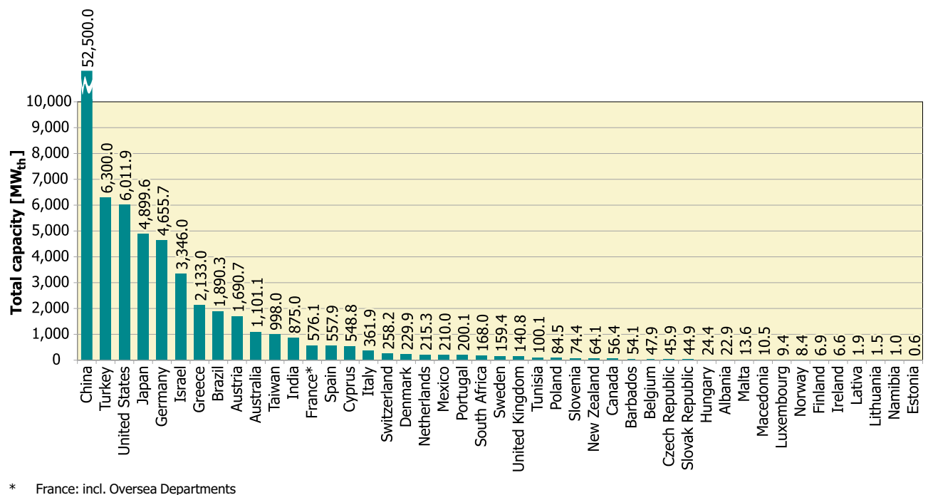
Figure 5: Total capacity of glazed flat plate and evacuated tube collectors in operation at the end of 2005
