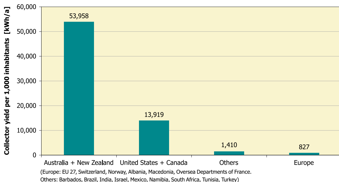
Figure 18: Annual collector yield of unglazed collectors in operation by economic region at the end of 2005 per 1,000 inhabitants
