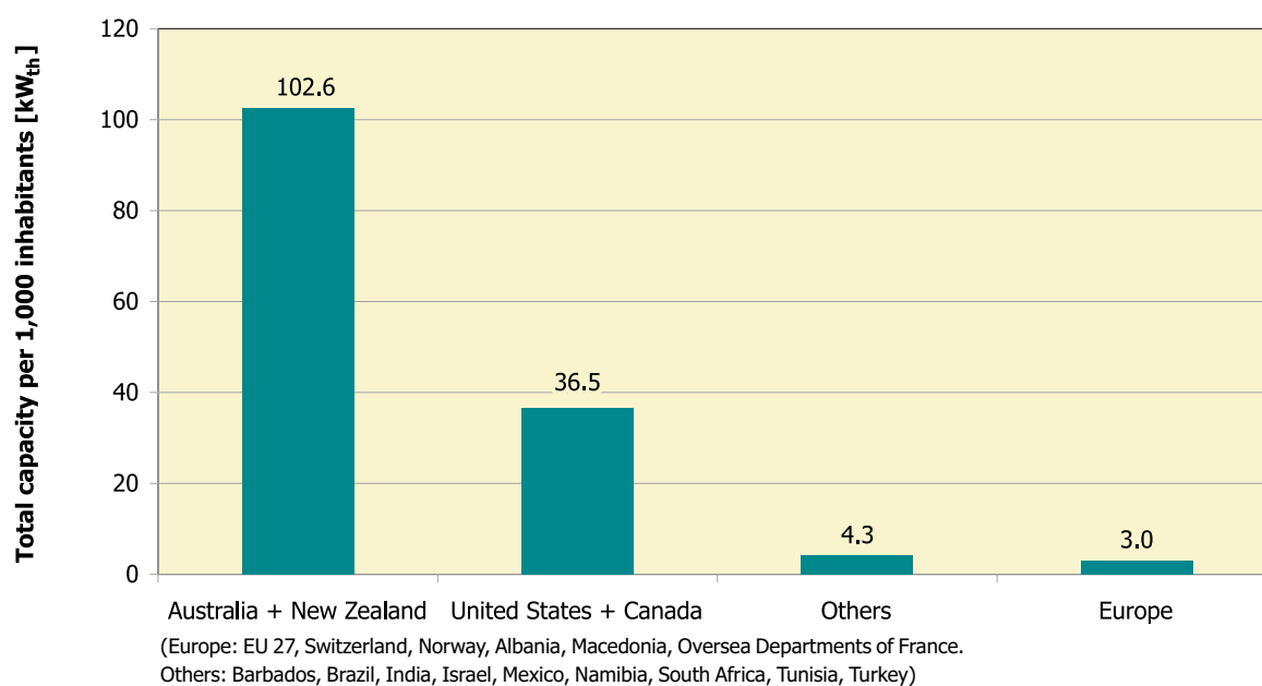
Figure 12: Total capacity of unglazed collectors in operation by economic region at the end of 2005 in \text{kW}_{\text{th}} per 1,000 inhabitants
