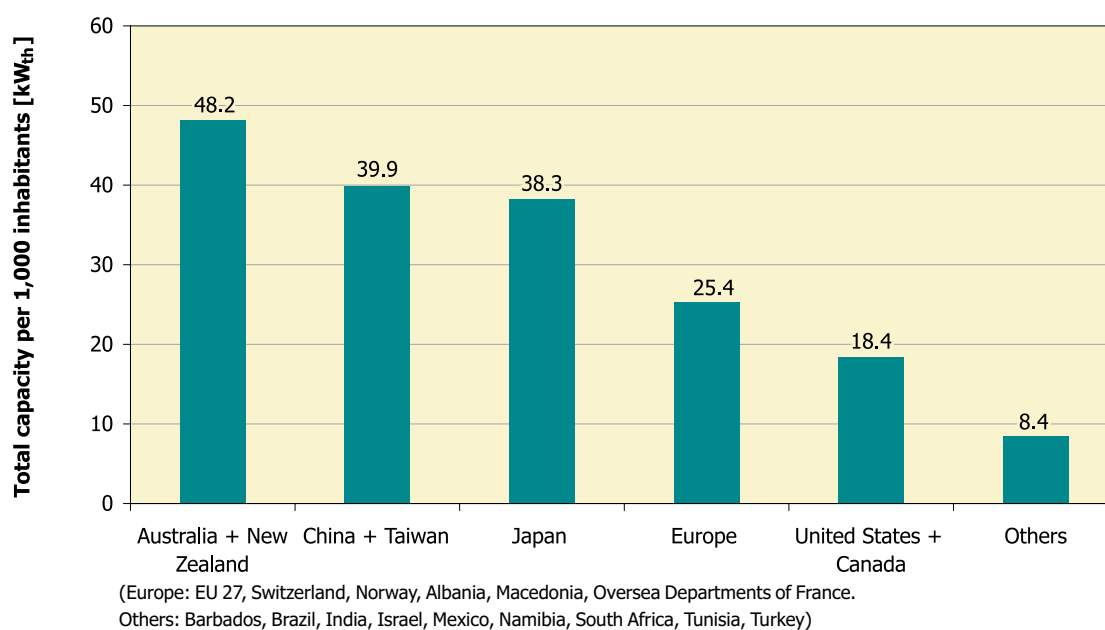
Figure 8: Total capacity of glazed flat plate and evacuated tube collectors in operation by economic region at the end of 2005 in kW th per 1,000 inhabitants
