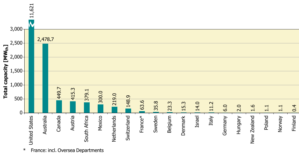
Figure 9: Total capacity of unglazed water collectors in operation at the end of 2005
