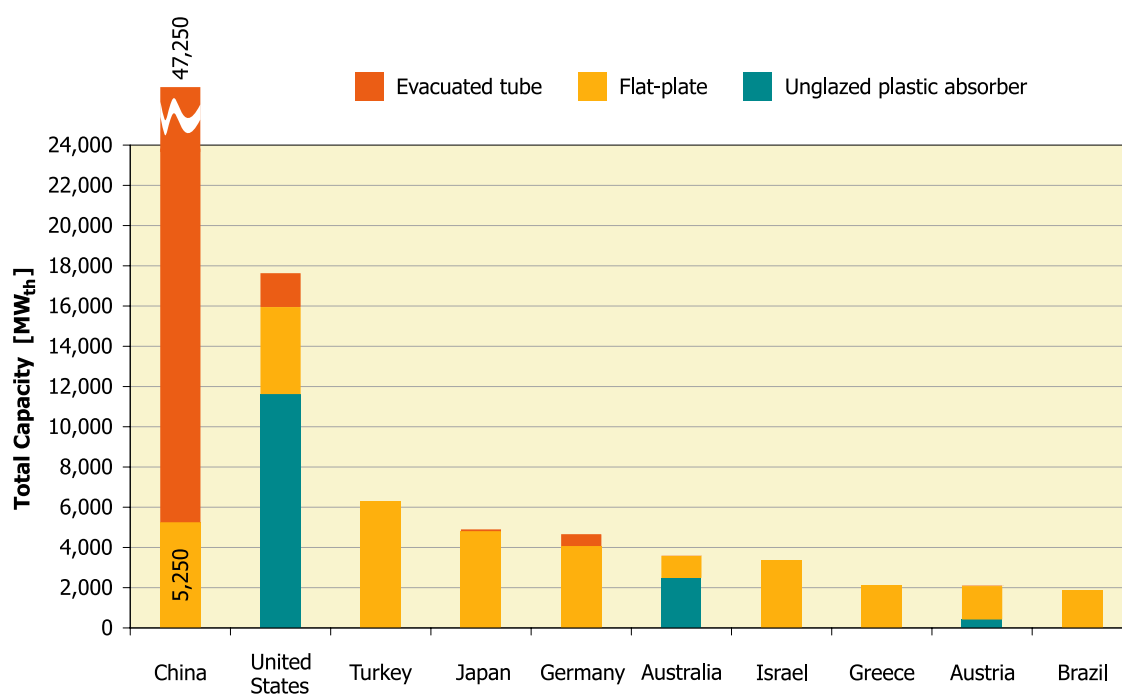
Figure 4: Total capacity in operation of water collectors of the 10 leading countries at the end of 2005
