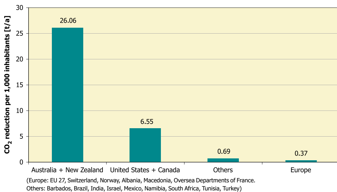
Figure 26: Annual contribution to CO 2 reduction by economic region at the end of 2005 per 1,000 inhabitants – unglazed collectors
