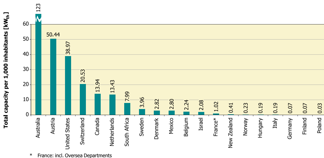
Figure 10: Total capacity of unglazed water collectors in operation at end of 2005 in \text{kW}_{\text{th}} per 1,000 inhabitants
