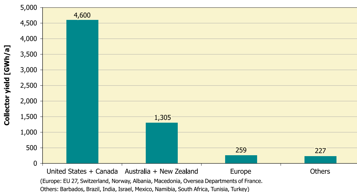
Figure 17: Annual collector yield of unglazed collectors in operation by economic region at the end of 2005
