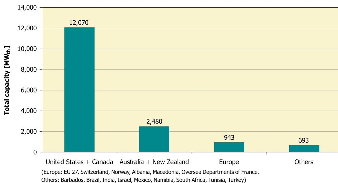
Figure 11: Total capacity of unglazed collectors in operation by economic region at the end of 2005
