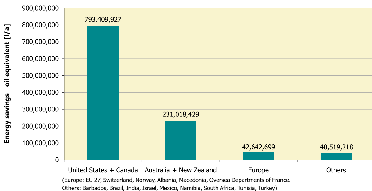
Figure 21: Annual energy savings in oil equivalent – unglazed collectors by economic region at the end of 2005
