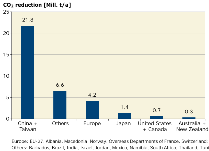
Figure 24: Annual contribution to CO 2 reduction by flat-plate and evacuated tube collectors by economic region the end of 2007
