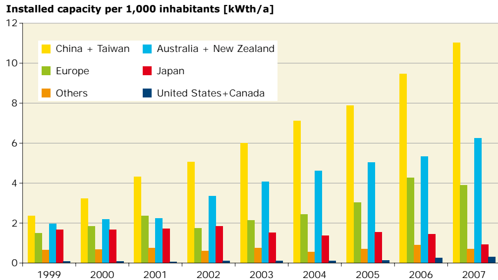
Figure 14: Annual installed capacity of flat-plate and evacuated tube collectors in kW th per 1,000 inhabitants from 1999 to 2007
