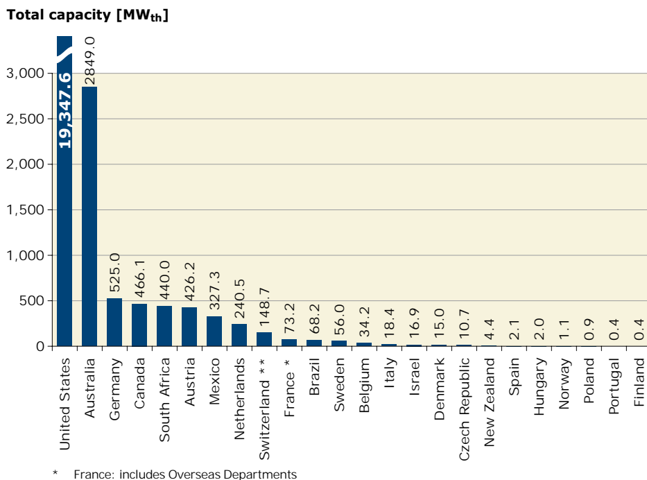
Figure 9: Total capacity of unglazed water collectors in operation at the end of 2007
