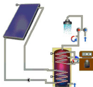
Figure 35: Hydraulic scheme of the DHW system for multi family houses
