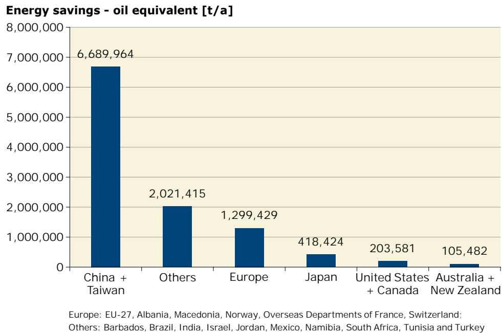
Figure 20: Annual energy savings in oil equivalent by glazed flat-plate and evacuated tube collectors by economic region at the end of 2007
