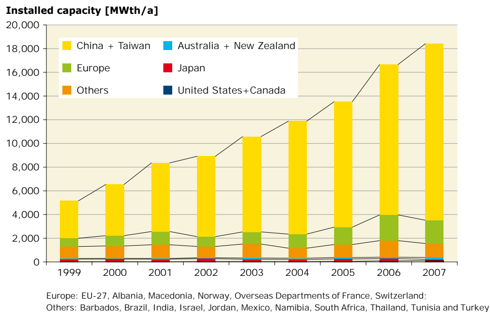
Figure 13: Annual installed capacity of flat-plate and evacuated tube collectors from 1999 to 2007
