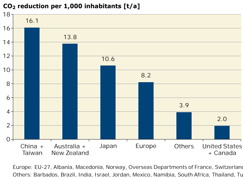
Figure 25: Annual contribution to CO 2 reduction by flat-plate and evacuated tube collectors by economic region at the end of 2007 per 1,000 inhabitants
