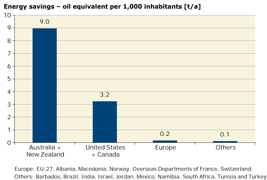
Figure 23: Annual energy savings in oil equivalent by unglazed collectors by economic region at the end of 2007 per 1,000 inhabitants
