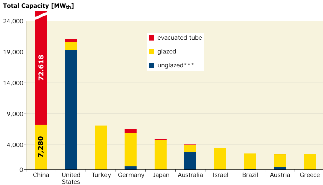
Figure 4: Total capacity in operation of water collectors of the 10 leading countries at the end of 2007
