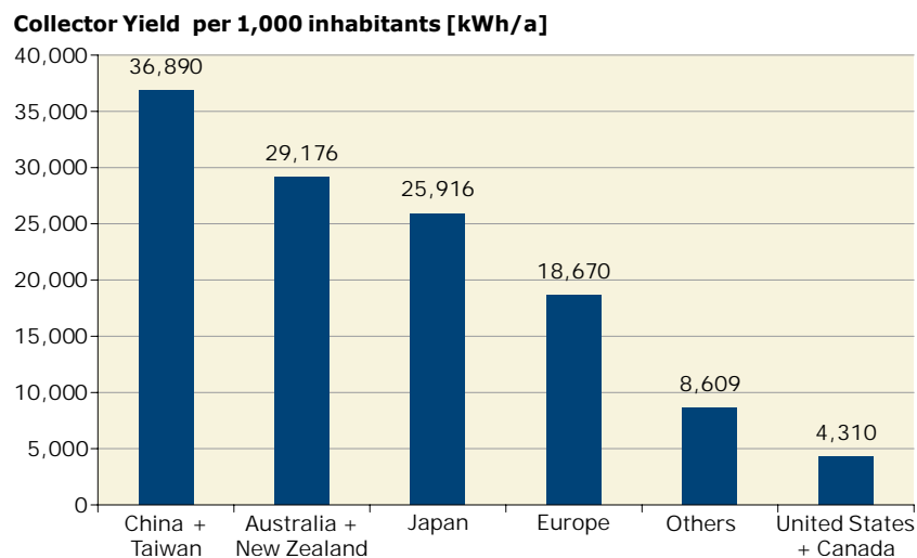
Figure 17: Annual collector yield of glazed flat-plate and evacuated tube collectors in operation by economic region at the end of 2007 in kWh per 1,000 inhabitants
