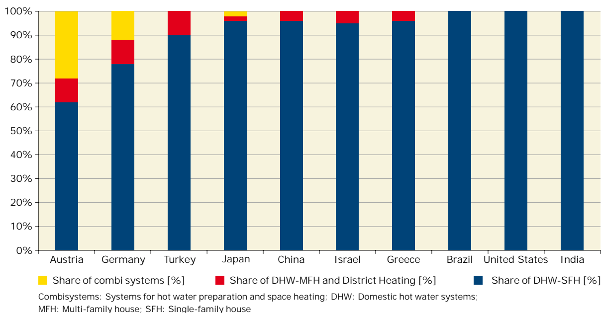
Figure 29: Distribution of different applications of the world's top-10-countries related to the total capacity in operation of glazed and evacuated tube collectors in 2007
