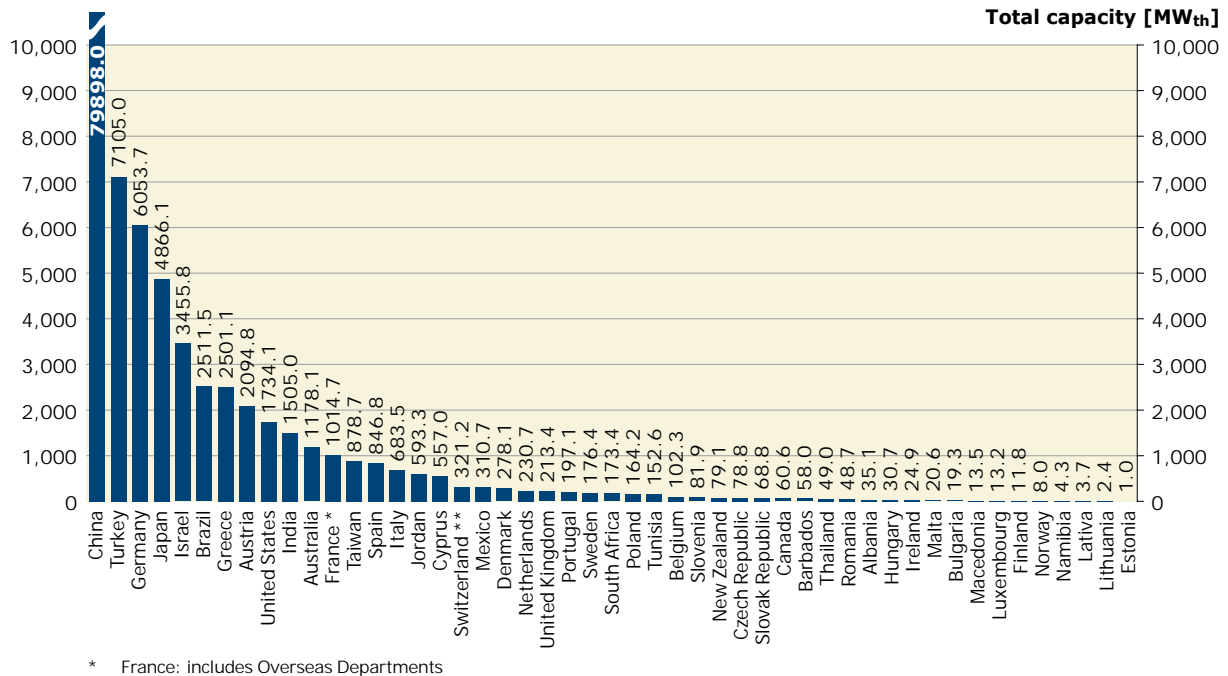
Figure 5: Total capacity of glazed flat-plate and evacuated tube collectors in operation at the end of 2007
