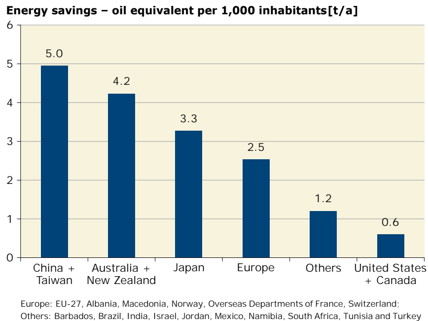
Figure 21: Annual energy savings in oil equivalent by glazed flat-plate and evacuated tube collectors in operation by economic region at the end of 2007 per 1,000 inhabitants
