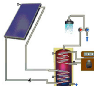
Figure 34: Hydraulic scheme of the DHW reference system
