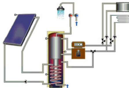
Figure 36: Hydraulic scheme of the solar combi reference system
