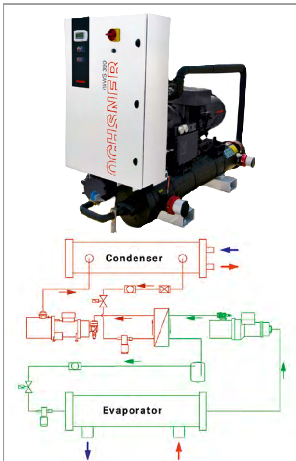
Standard industrial heat-pump (water)/two-stage cycle process Source: Ochsner Wärmepumpen GmbH
