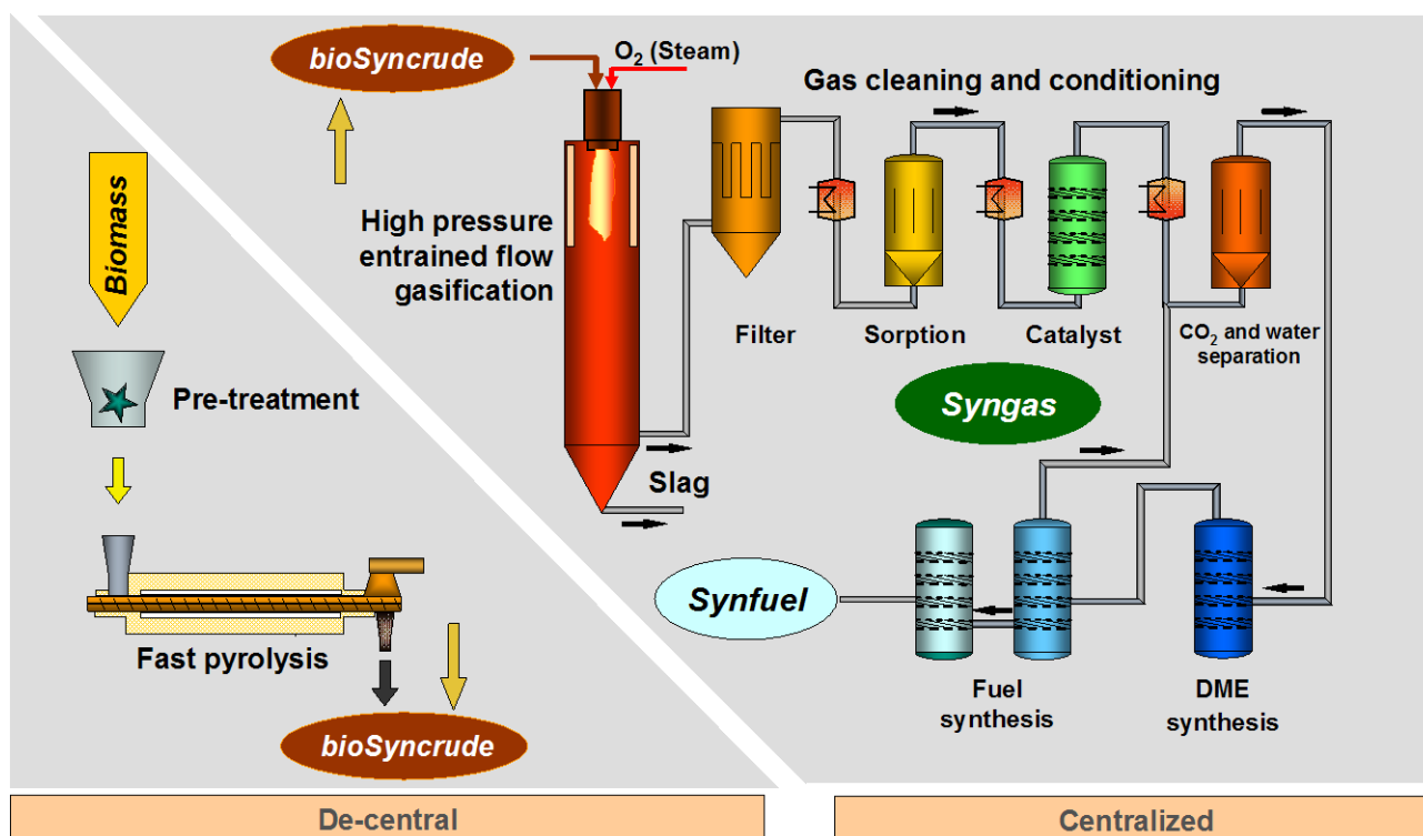
Figure 4. Technology scheme of the de-central/centralized bioliq concept
