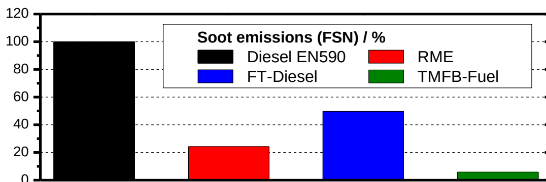
Figure 3. Soot emissions of different biofuels
