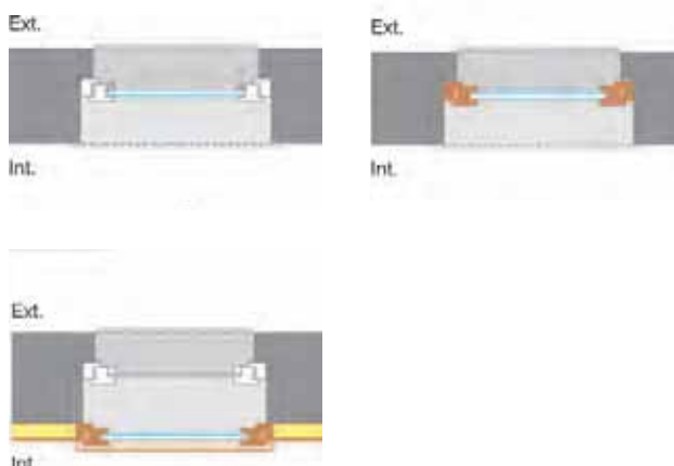
↑ Illustration 203 : Conservation of existing openings
