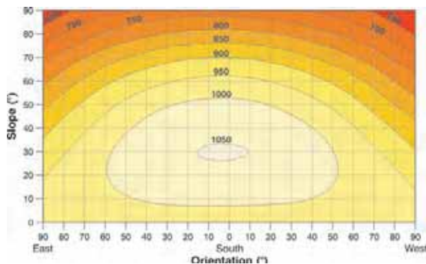
↑ Illustration 317 : Influence of the orientation and slope on the efficiency
