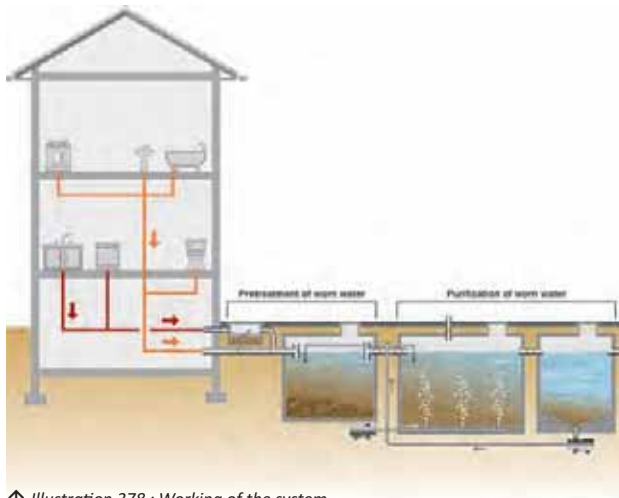
↑ Illustration 378 : Working of the system
