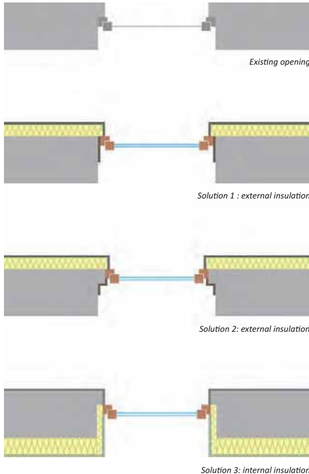
↑ Illustration 202: Modification of existing openings - Various solutions
