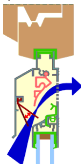
↑ Illustrations 92 and 93: Grilles for air intake in new frames
