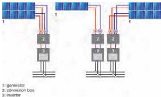
↑ Illustration 315 : Various types of inverter installation
