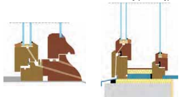
↓ Illustration 208 : Mobile overglazing of the existing window
