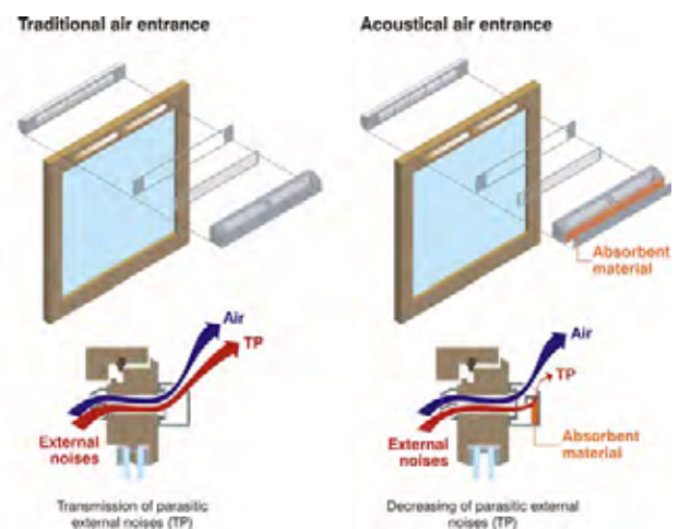
↑ Illustration 112 : Principle of acoustical air entrance
