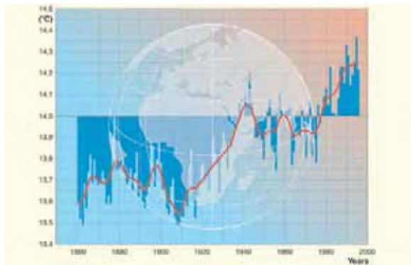
↑ Illustration 416 : Global Warming since 1860
