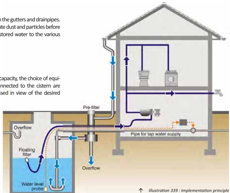
↑ Illustration 339 : Implementation principle
