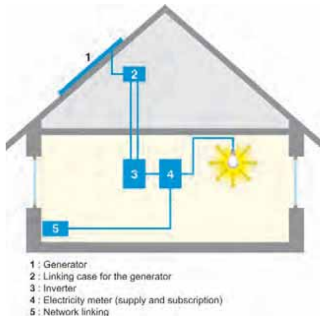
↑ Illustration 307 : Installation diagram
