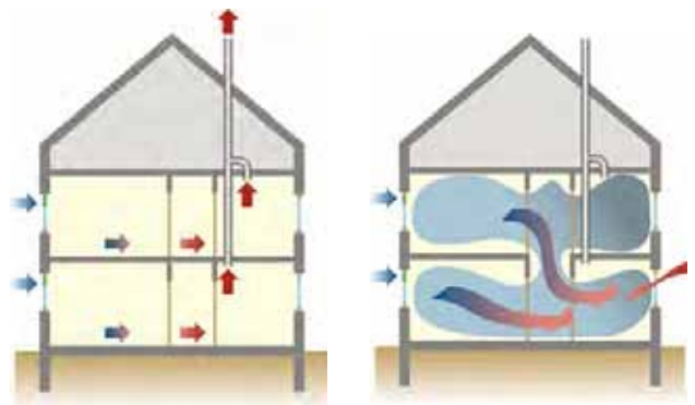
↑ Illustration 86: System B: Ventilation single flow
