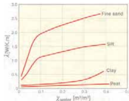
↑ Illustration 332: Nature of different type of grounds
