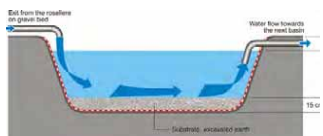
↑ Illustration 370 : Plankton basin
