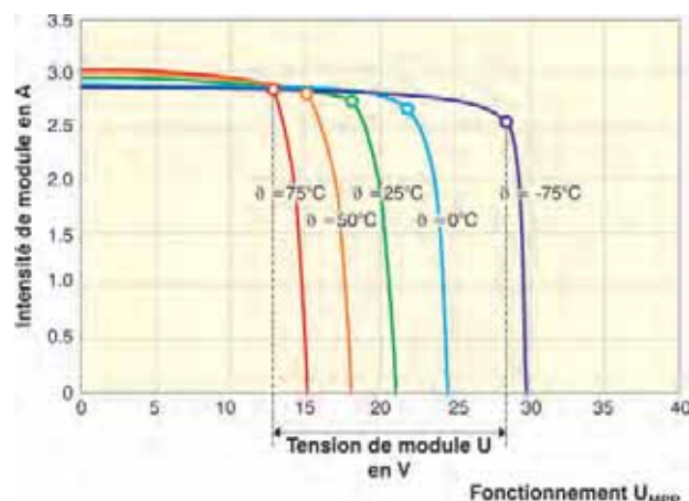
↑ Illustration 313 : Impact or influence of temperature
