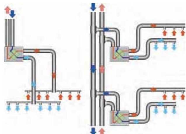
↑ Illustration 325 : Implementation of an heat recovery system in individual housing
