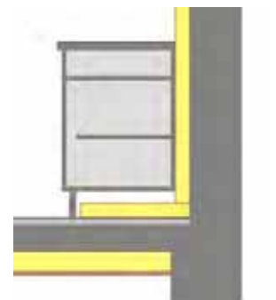
↑ Illustration 153 : Insulation by inside (floor and wall)
