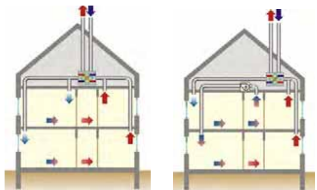
↑ Illustration 88: System D: Balance ventilation system
