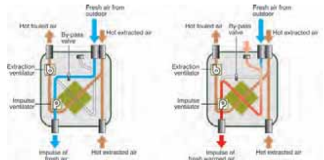
↑ Illustration 324 : Working of a heat recovery system
