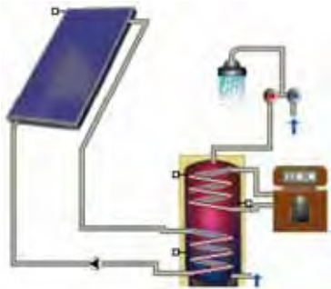
Figure 44: Hydraulic scheme of the domestic hot water pumped reference system for single family houses
