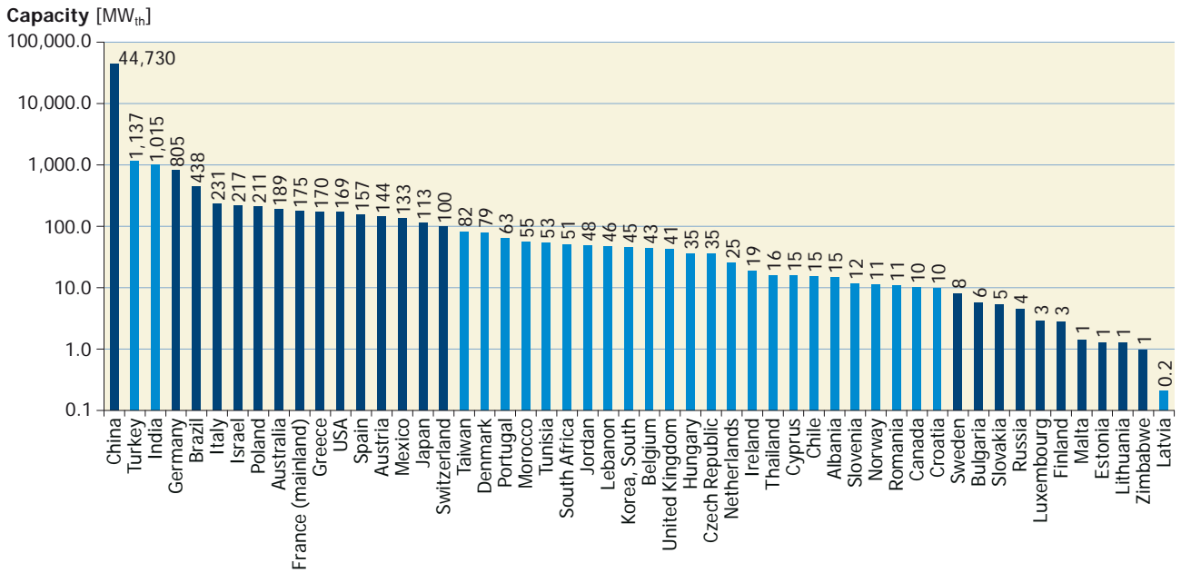
Figure 20: Newly installed capacity of glazed water collectors in 2012
