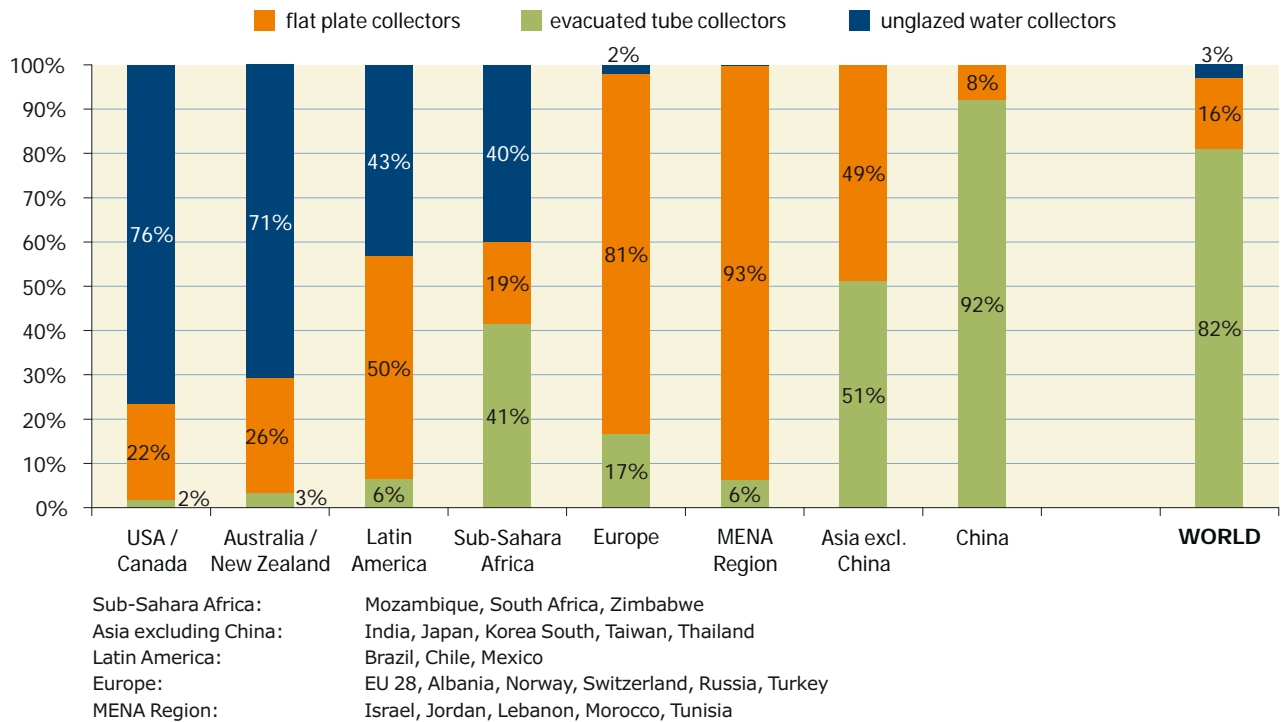
Figure 34: Distribution by type of solar thermal collector for the newly installed water collector capacity in 2012
