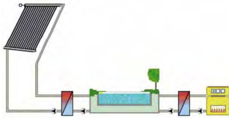
Figure 43: Hydraulic scheme of the swimming pool reference system
