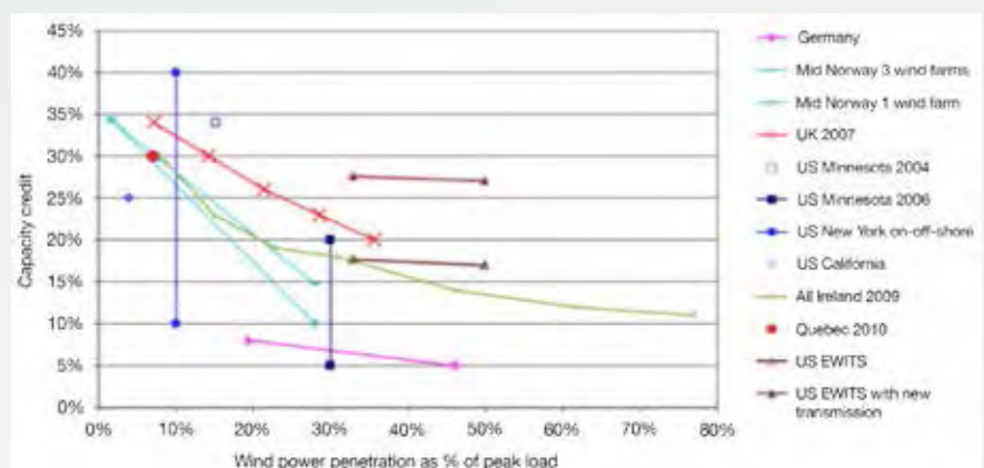
Figure 2. Capacity credit of wind power. Results from ten studies show reduction of capacity value as penetration level increases. New York on- and offshore shows the range of capacity value for wind, when calculated only for onshore sites (10%) or only offshore sites (40%).
