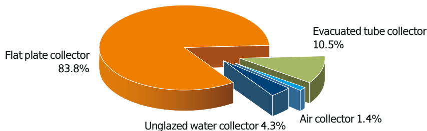
Figure 7: Distribution of the total installed capacity in operation by collector type in 2013 – EUROPE
