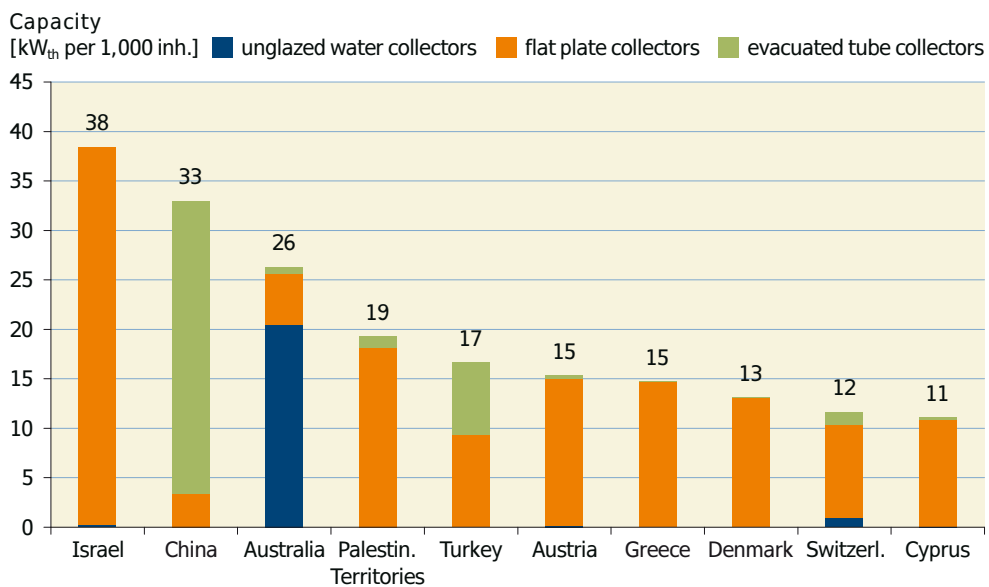
Figure 21: Top 10 markets for glazed and unglazed water collectors in 2013 (relative figures in kW th per 1,000 inhabitants)
