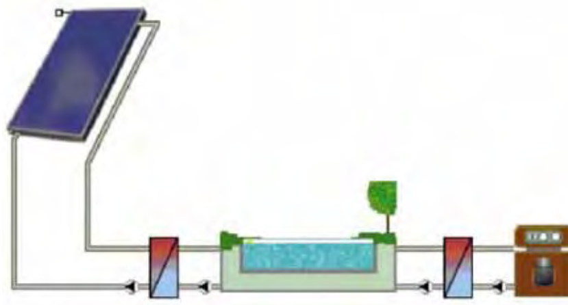
Figure 44: Hydraulic scheme of the swimming pool reference system
