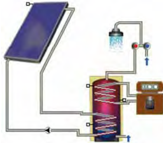
Figure 45: Hydraulic scheme of the domestic hot water pumped reference system for single family houses
