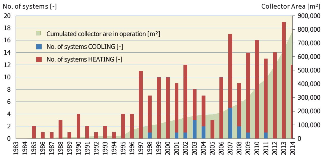
Figure 40: Solar district heating and cooling in Europe – annual achievements and cumulated area in operation by end of 2014 (Data source: Jan-Olof Dalenbäck - Chalmers University of Technology, SE)
