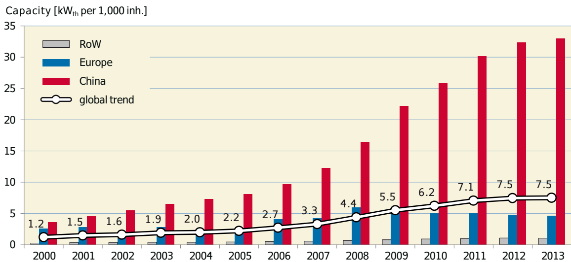
Figure 28: Annual installed capacity of glazed water collectors in kW th per 1,000 inhabitants from 2000 to 2013
