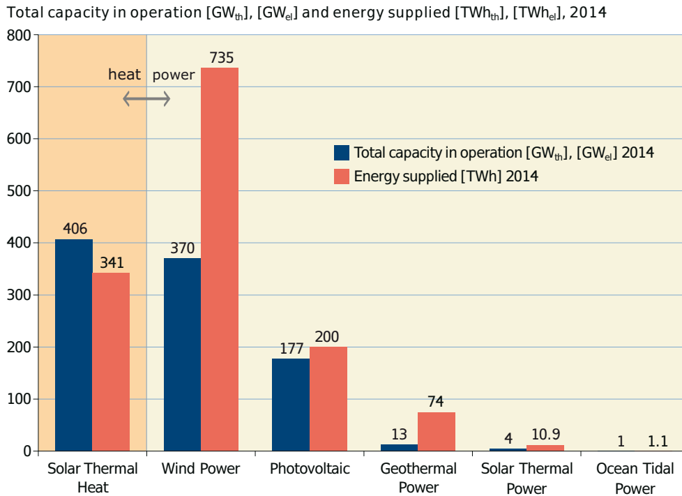
Figure 3: Global capacity in operation [GW el ], [GW th ] 2014 and annual energy yields [TWh el ], [TWh th ] (Sources: AEE INTEC, Global Wind Energy Council (GWEC), European PV Industry Association (EPIA), REN21 - Global Status Reports 2014 and 2015)
