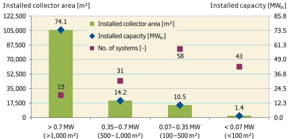
Figure 43: Global solar process heat applications in operation (Source: IEA SHC Task49/IV SHIP database)
