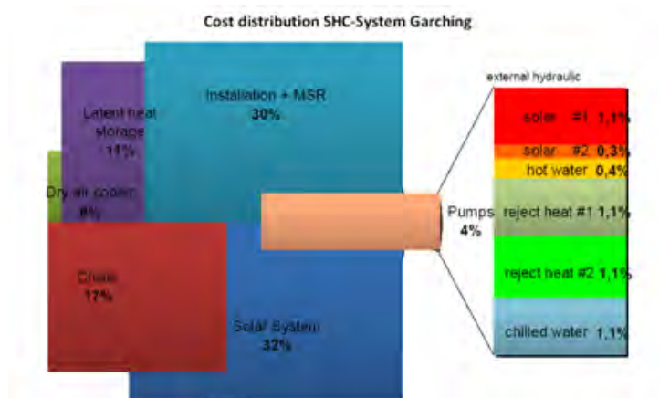
Figure 4. Cost distribution for SHC System Garching.
