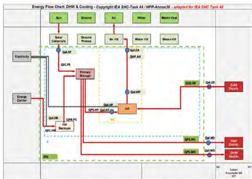
Figure 9: system boundary and possible energy flows for the SPF_{el,sys}
