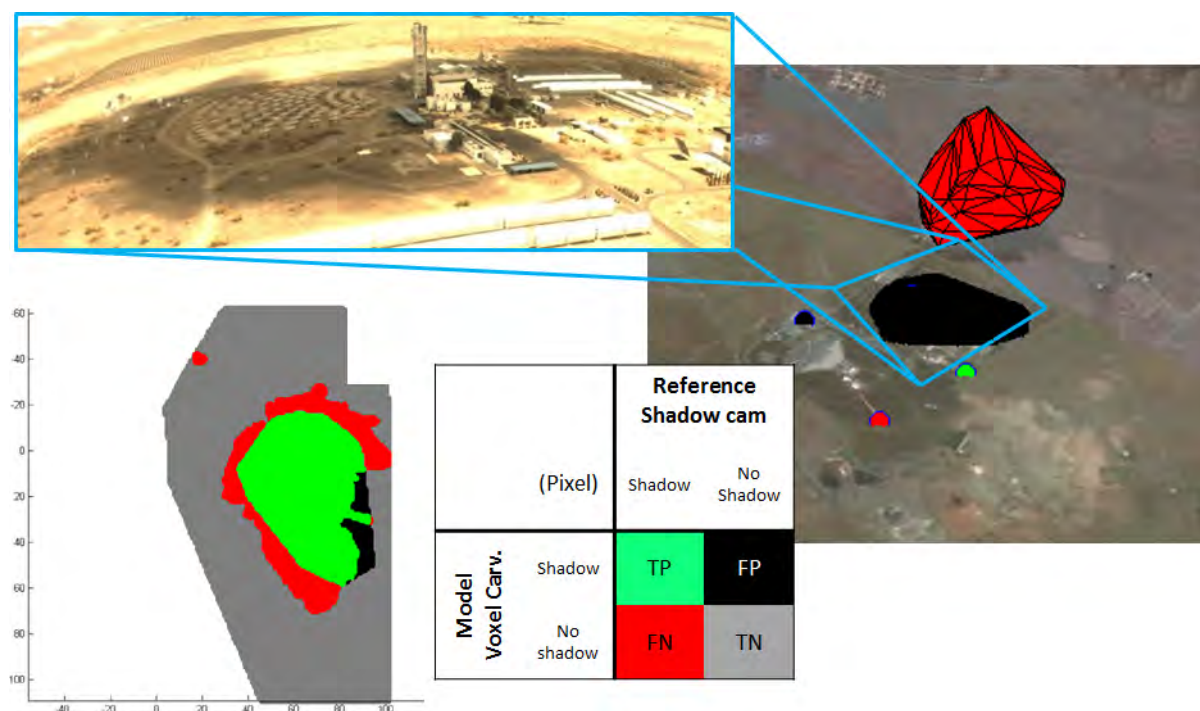
Figure C2. Comparison of cloud shadow derived from four all sky imagers (right) and “shadow-cameras” (left) (Oberländer et al., 2015).
