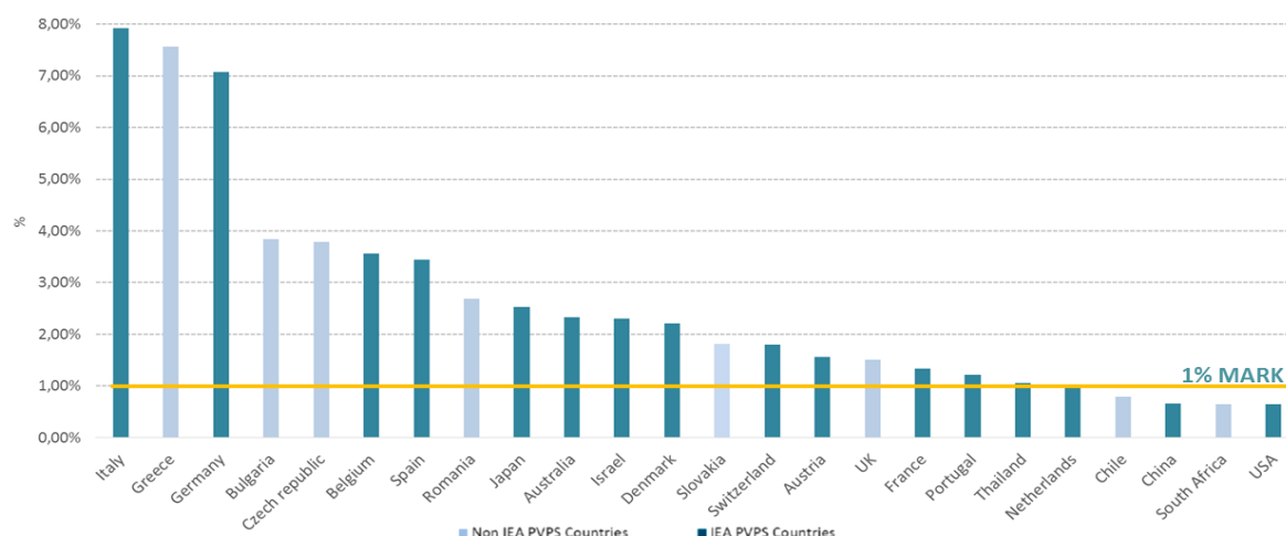
FIGURE 4: 2014 THEORETICAL PV PRODUCTION
