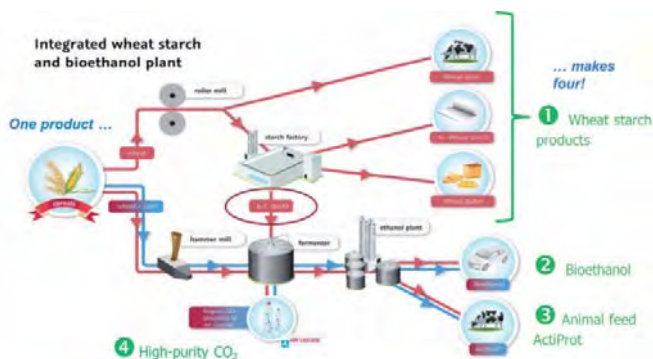
Figure 16. Agrarian raw materials biorefinery facility Pischelsdorf, Austria [AGRANA]
