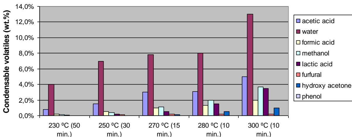
Figure 5-1 Composition of volatiles released during torrefaction of willow at different temperatures (Prins, 2005)
