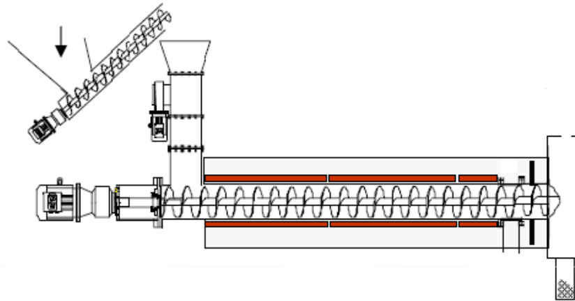
Figure 3-2 Auger screw type reactor
