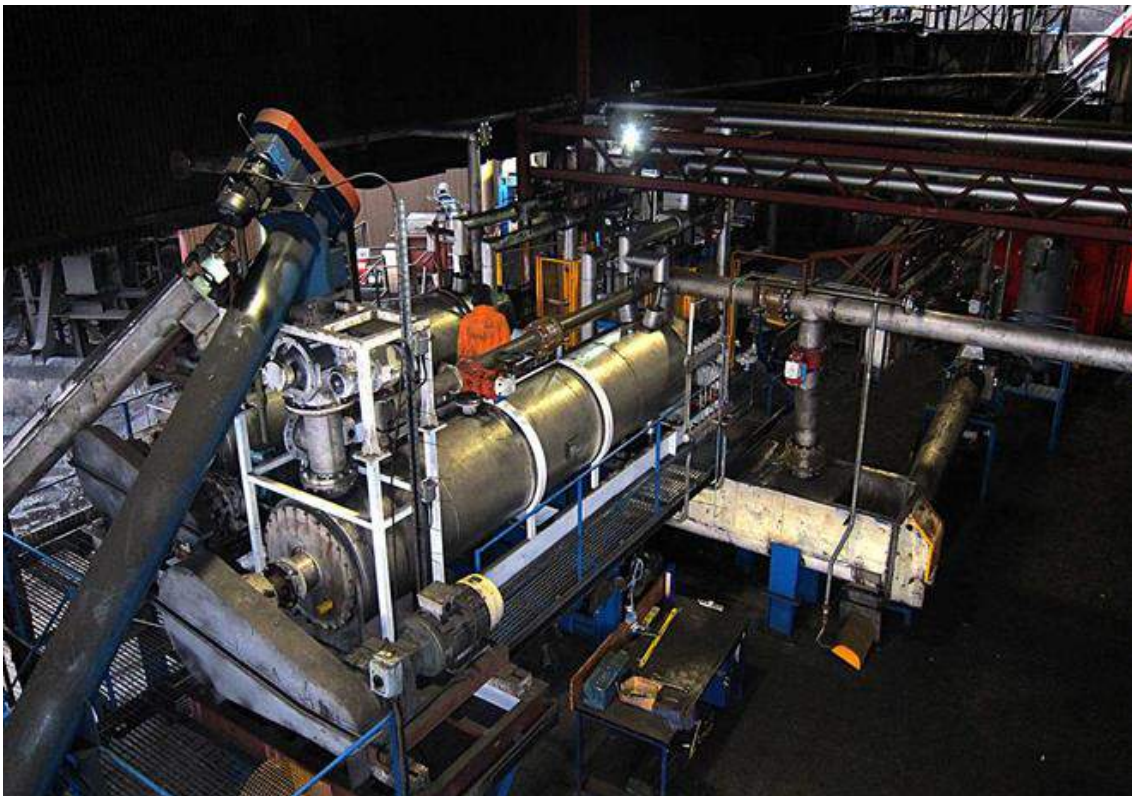
Figure 4-11 Modified screw reactor of Arigna Fuels.
