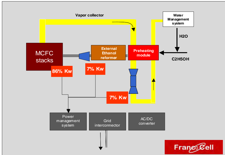
Figure 8 – The Franco Cell solution: a multimegawatt power unit with 56% electrical efficiency from ethanol as fuel and “zero” NO x , SO 2 and particulates [source: FrancoCell, presentation at IWMC 2012, Paris]
