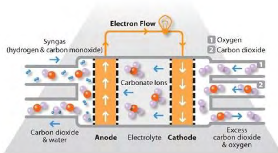
Figure 1 – Schematic representation of the operation of an MCFC [source: www.fuelcelltoday.com ]
