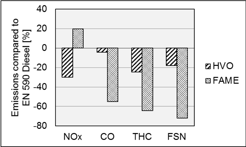
Fig.2 Reduction of Emissions with the Use of HVO and FAME
