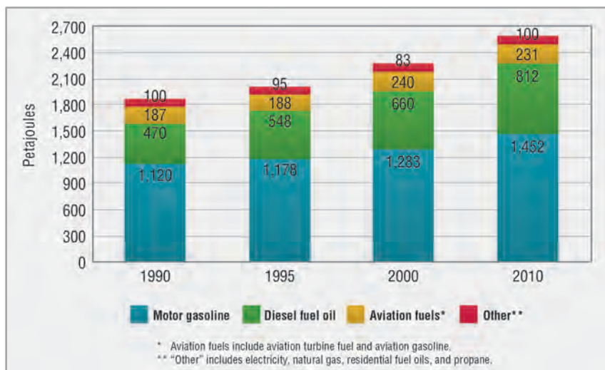
Fig. 4 Transportation Sector Energy Use by Energy Source in Selected Years (Source: http://oee.nrcan.gc.ca/corporate/statistics/neud/dpa/data_e/trends.cfm?attr=0 )
