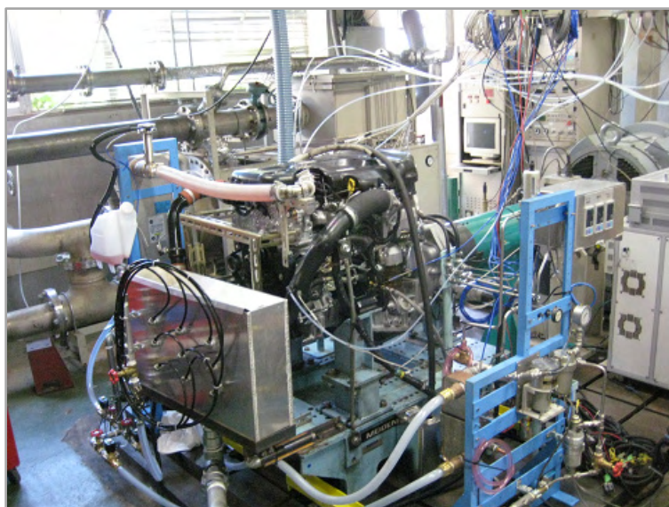
Fig. 2 Test Engine
