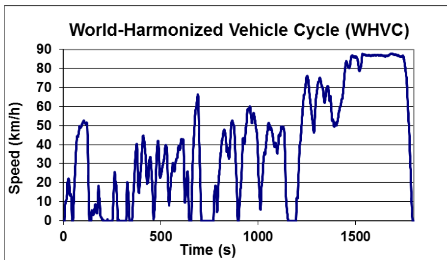
Fig. 1 World Harmonized Vehicle Cycle
