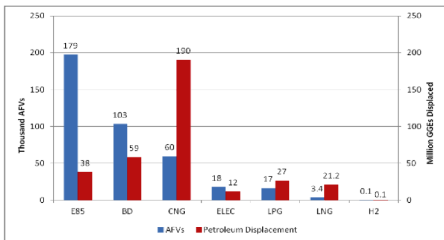
Fig. 1 Clean Cities 2012 Data for Advanced Fuel Vehicles (AFVs) and Petroleum Displacement 36
