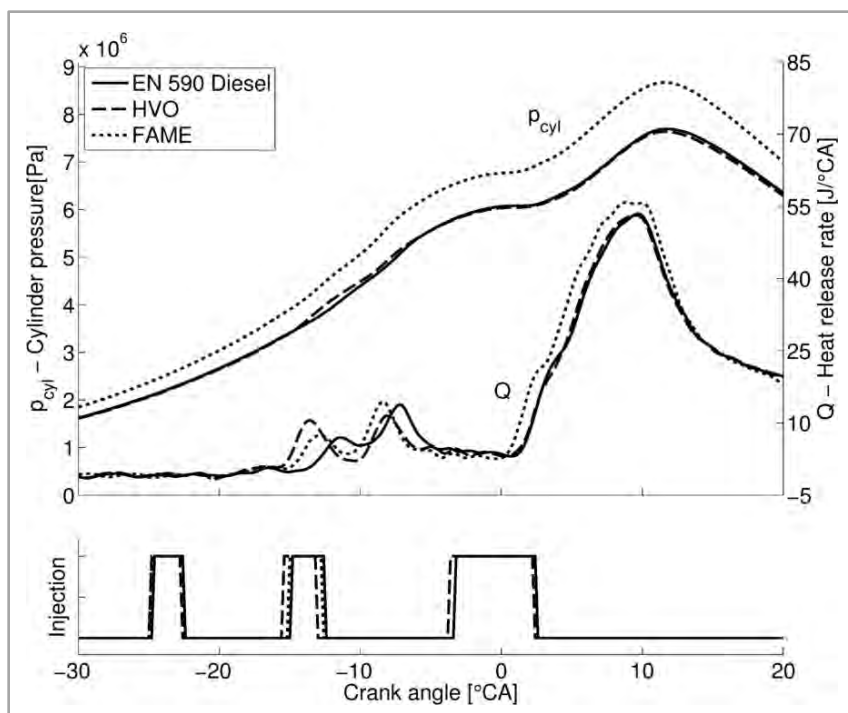
Fig. 1 Cylinder Pressure, Heat Release Rate, and Injection for HVO, FAME, and Reference Diesel (EN 590), n = 2,000\text{min}^{-1} , p_{me} = 9 bar
