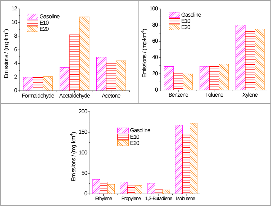
Fig. 1 NEDC: Unregulated Pollutant Emissions (ethanol fuels at -7°C)
