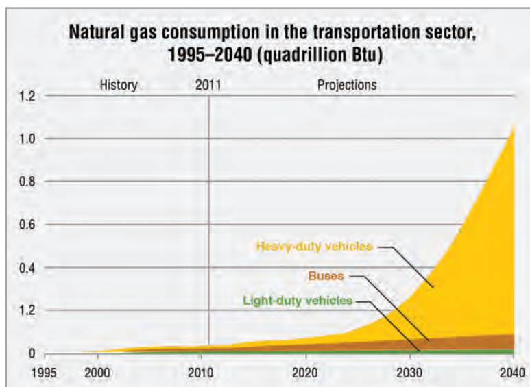
Fig. 3 Consumption of Natural Gas by Light- and Heavy-Duty Vehicles and Buses for the Period 1995–2040
