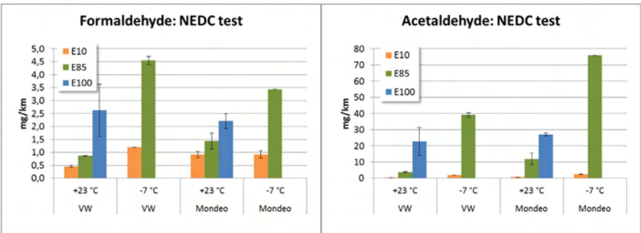
Fig. 2 Cold-Start NEDC: Unregulated Pollutant Emissions (ethanol fuels)
