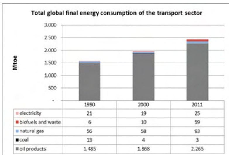
Fig. 2 Total Global Final Energy Consumption of the Transport Sector (IEA Statistics)
