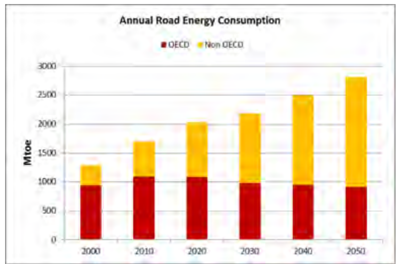
Fig. 4 Global Annual Road Energy Consumption Projections (IEA Energy Technology Perspectives 2012)
