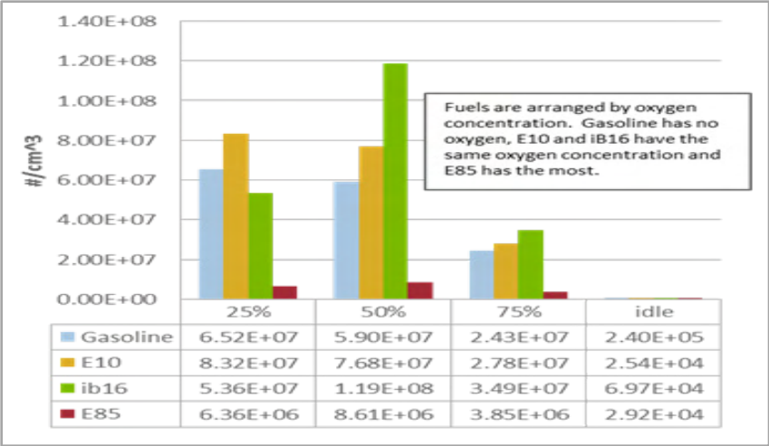
Fig. 2 Total Particulate Concentrations ( \#/cm^3 ): 2.2-Liter DISI Engine
