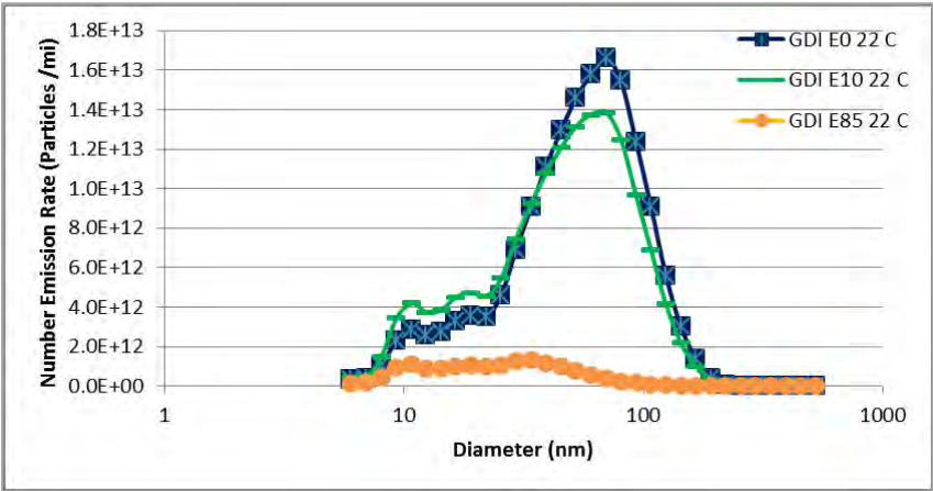
Fig. 3 Particle Size Distributions (mi) for DISI Vehicle Running on E0 and E85 over FTP-75 Driving Cycle
