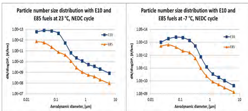
Fig. 4 Particle Size Distributions (/km) for DISI Vehicle Running on E10 and E85 over the NEDC at Various Ambient Temperatures
