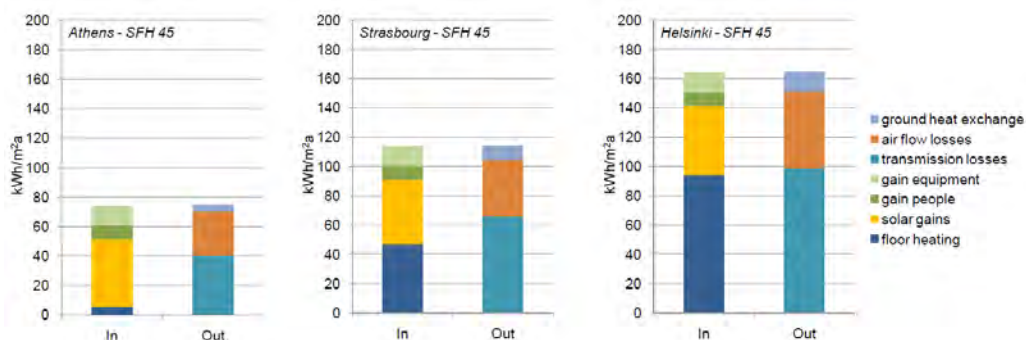
Figure 7: Building energy balances of a Single Family building with an annual heating demand of 45 kWh/(m²year) for Strasbourg climate - SFH 45 - at three different reference location.
