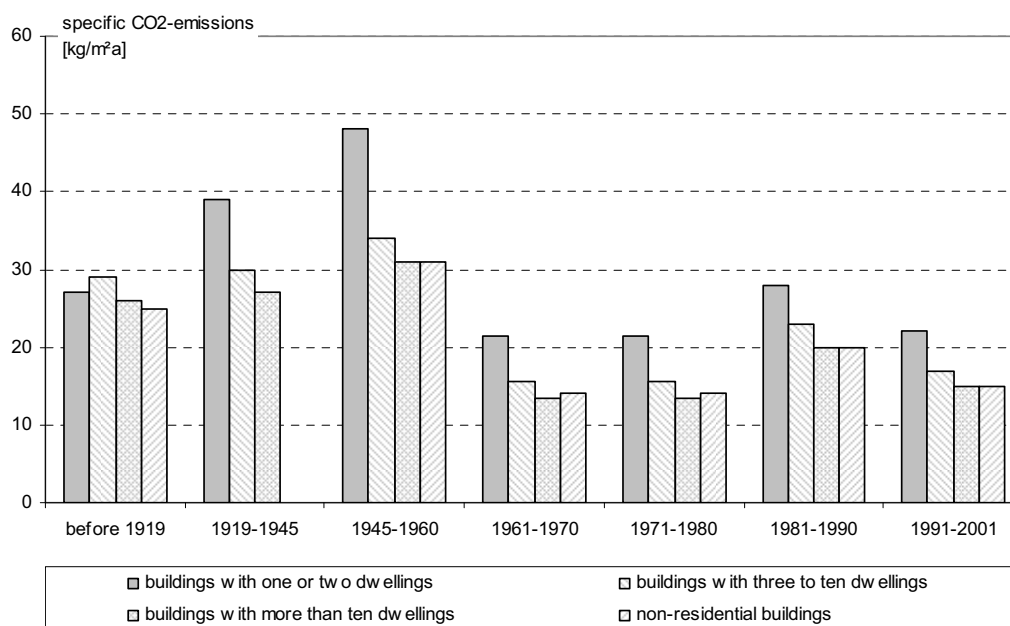
Fig. 11: Specific CO 2 -emissions of buildings with one or two dwellings, buildings with three to ten dwellings, buildings with more than ten dwellings and non-residential buildings in Austria classified by the building age. (data source: [Austrian Federal Economic Chamber 2006])
