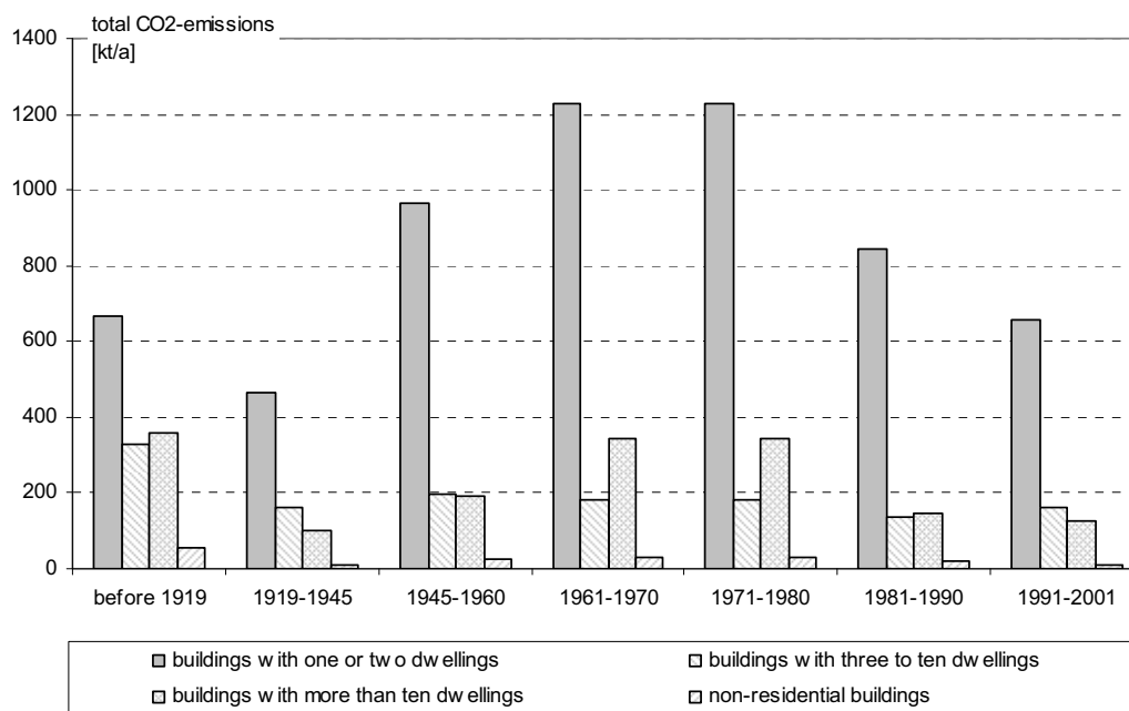
Fig. 10: Total CO 2 -emissions of buildings with one or two dwellings, buildings with three to ten dwellings, buildings with more than ten dwellings and non-residential buildings in Austria classified by the building age. (data source: [Austrian Federal Economic Chamber 2006])
