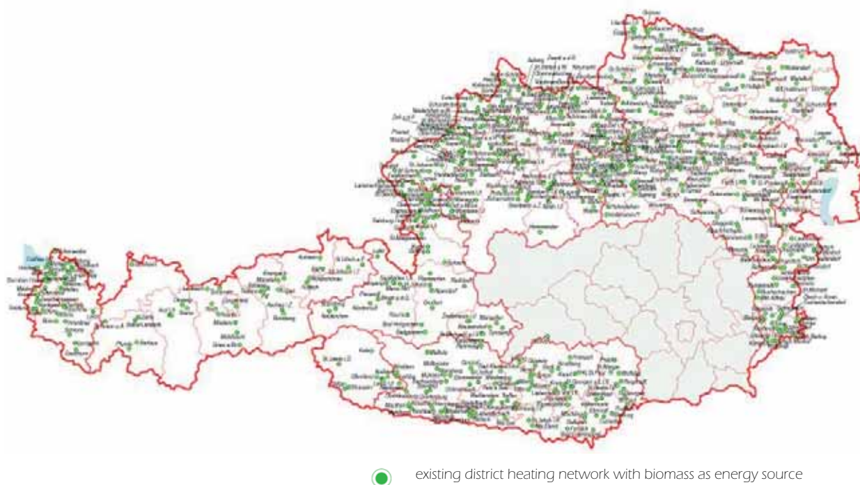
Fig. 24: District heating networks with biomass as energy source in Austria (except Styria, see Fig. 25). (data from December 2003; source: [LEV 2008a])
