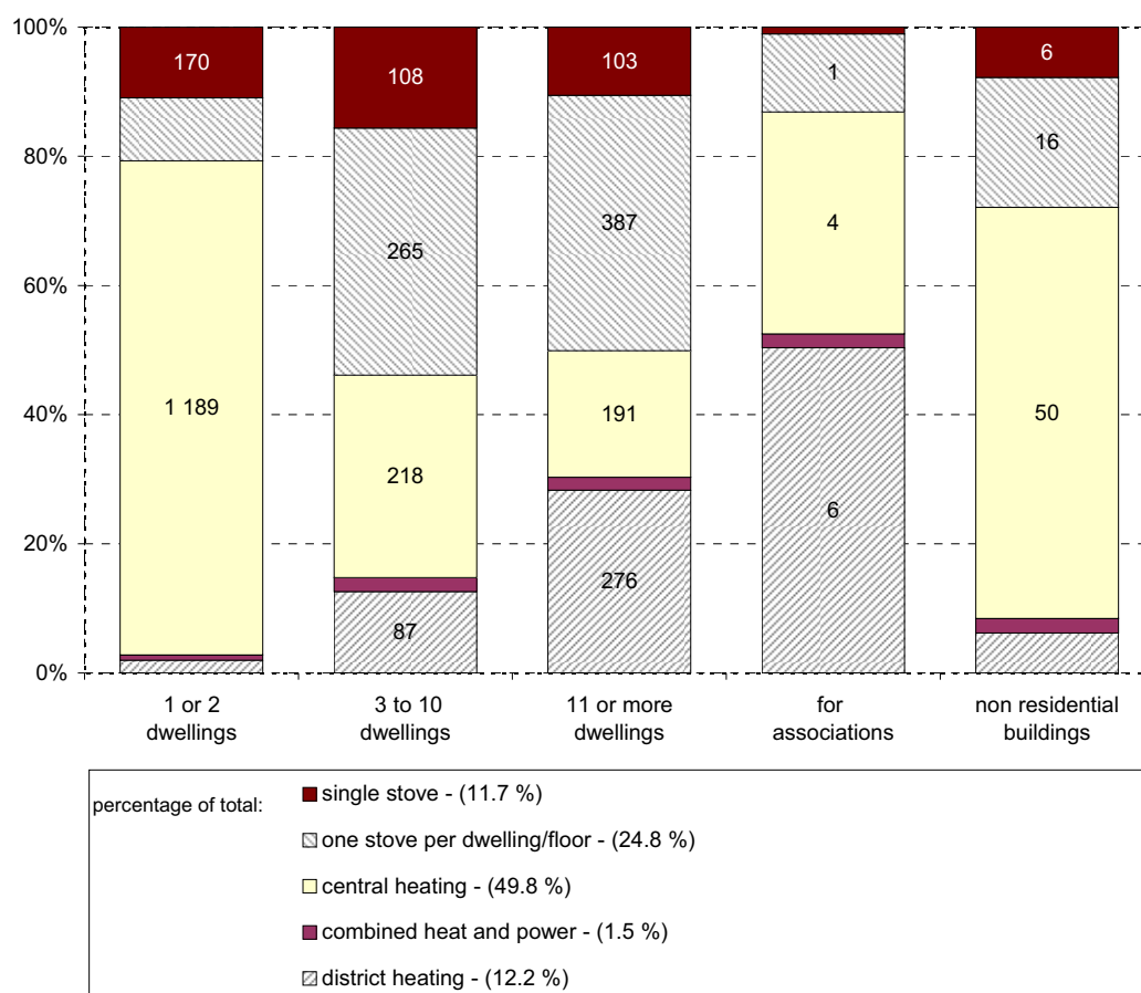
Fig. 8: Heat delivery systems in Austrian dwellings per building type in 2001. The figures inside the columns show the number of systems in 1000. (data source: [Statistics Austria 2007])
