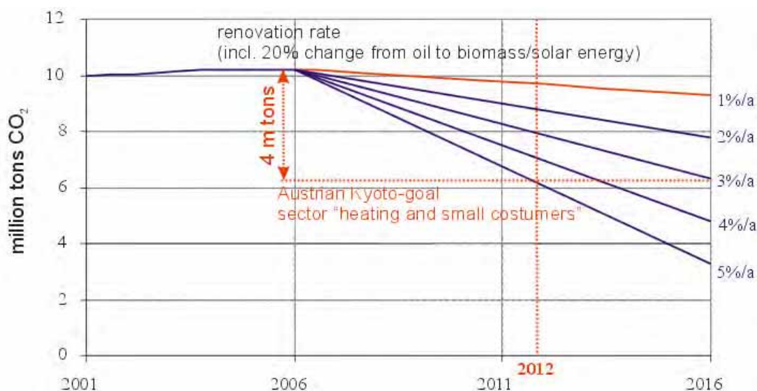
Fig. 18: Trend scenario of thermal renovation and fuel switch of all Austrian dwellings (origin figure: [Austrian Federal Economic Chamber, 2006], basic data from [Statistics Austria 2004])
