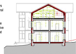
Section
