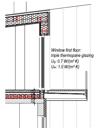
Window section – south terrace
