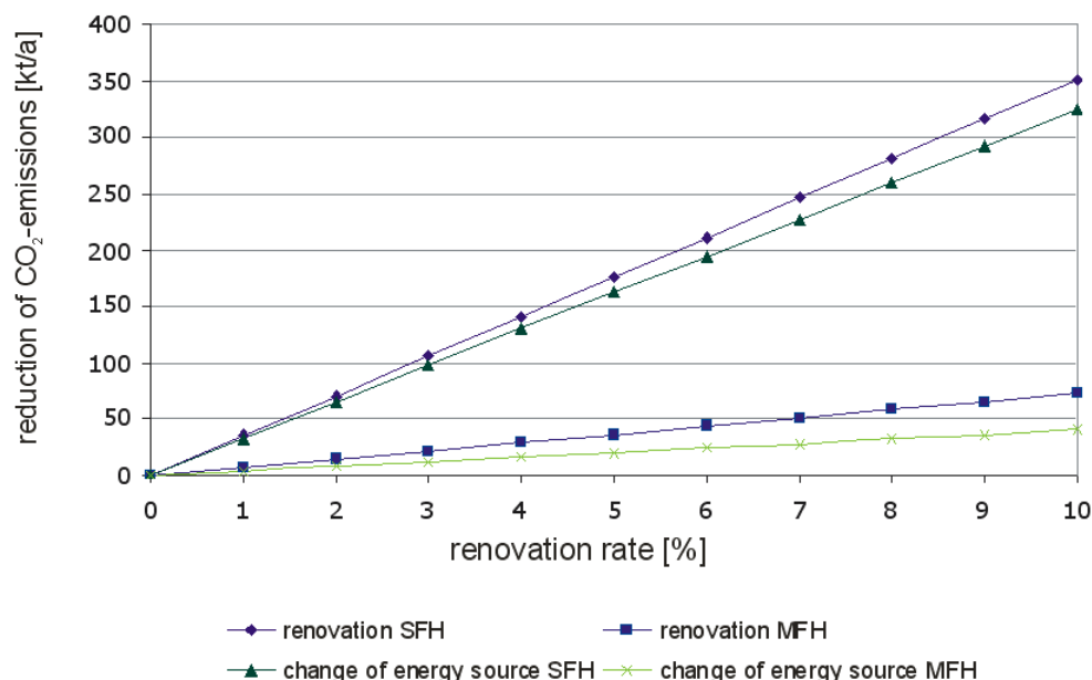
Fig. 17: Illustration of the potential for reduction of CO 2 -emissions due of single family buildings (SFH) and multi family buildings (MFH) due to a raise of the renovation rate and change of heating energy source to renewable energy (20 % change from oil to biomass/solar energy) for one- and multi-family dwellings [Austrian Federal Economic Chamber, 2006]
