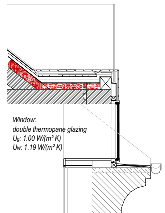
Window section
