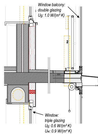
Window and terrace section
