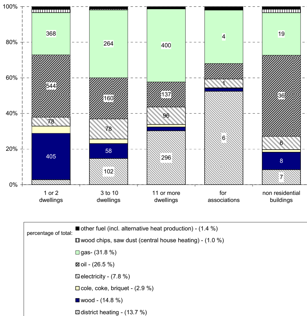
Fig. 9: Energy sources per building type for 3.32 mio Austrian dwellings. The figures in-side the columns show the number of systems in 1000. (data source: [Statistics Austria 2007])
