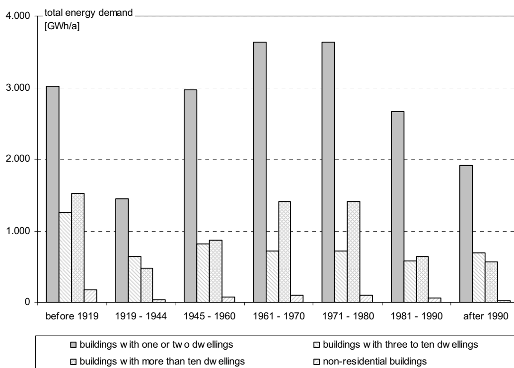
Fig. 7: Total energy demand of buildings with one or two dwellings, buildings with three to ten dwellings, buildings with more than ten dwellings and non-residential buildings in Austria classified by the building age. (data source: [Statistics Austria 2004], [Statistics Austria 2006], [Jungmeier et al. 1996])
