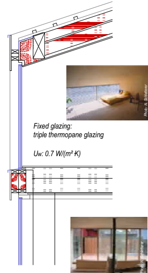
Window section
