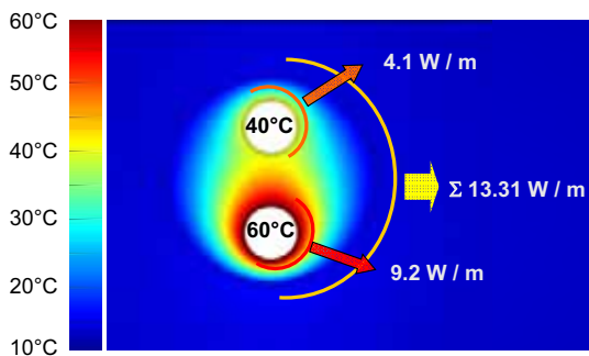
picture 12: Cross section of two pipes, enquiry of the thermal losses of the pipes in the supply network, image source [18]
