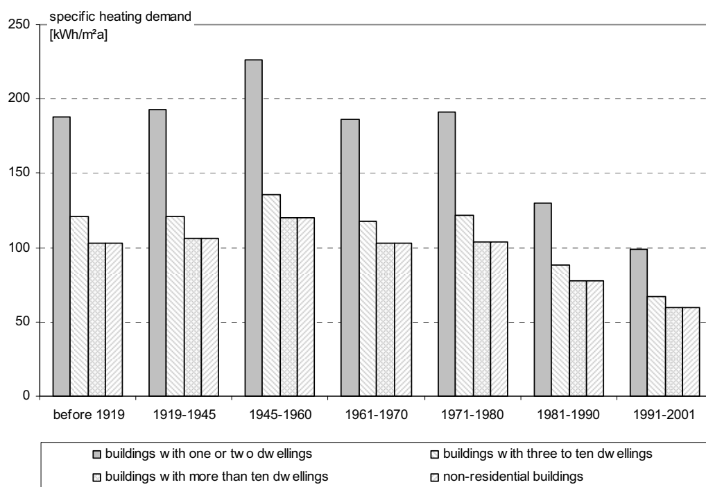
Fig. 6: Specific space heating energy demand (useful energy) of buildings with one or two dwellings, buildings with three to ten dwellings, buildings with more than ten dwellings and non-residential buildings in Austria classified by the building age. (data source: [Austrian Federal Economic Chamber 2006], origin data source: [Jungmeier et al. 1996])
