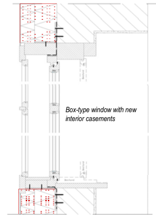
Window renovation – vertical section
