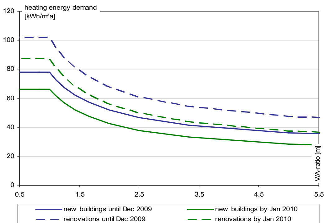
Fig. 21: Upper limits for heating energy demand of new buildings and renovations, (data source: [OIB 2007a])
