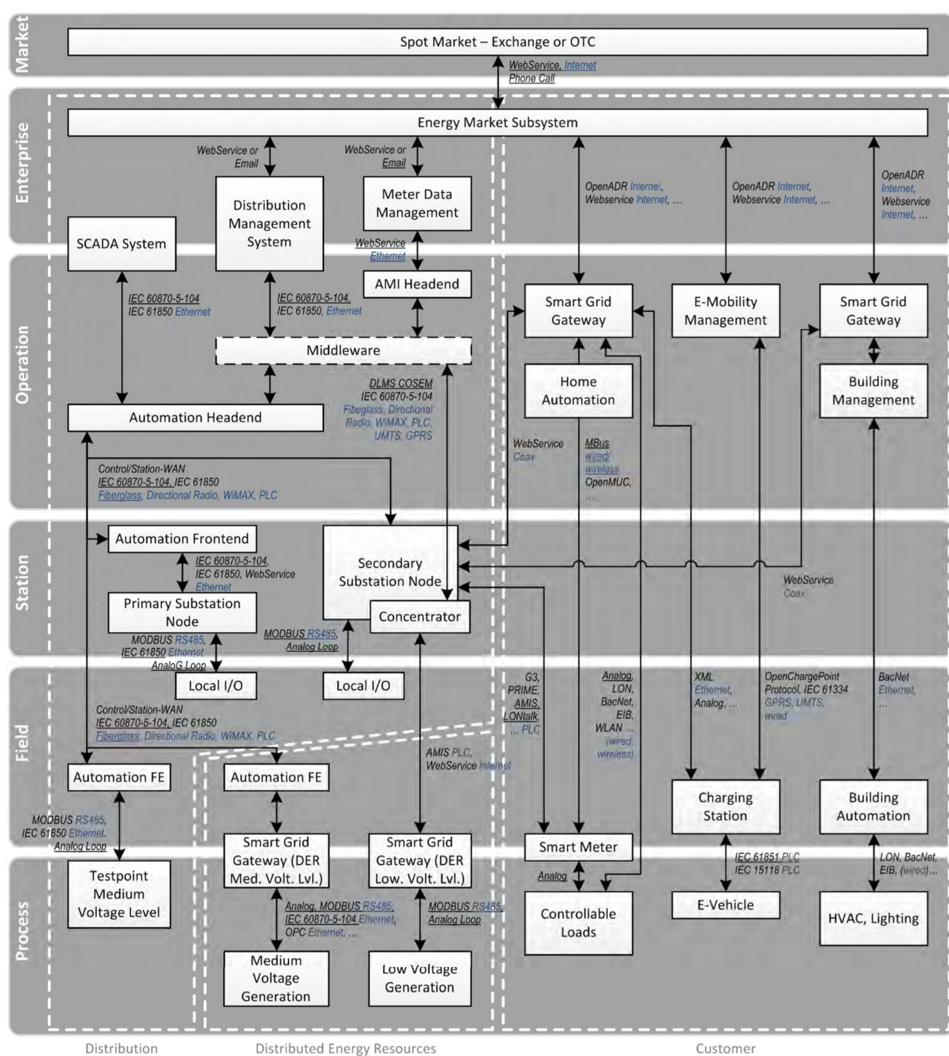
Fig. 1: (SG) 2 architecture model
