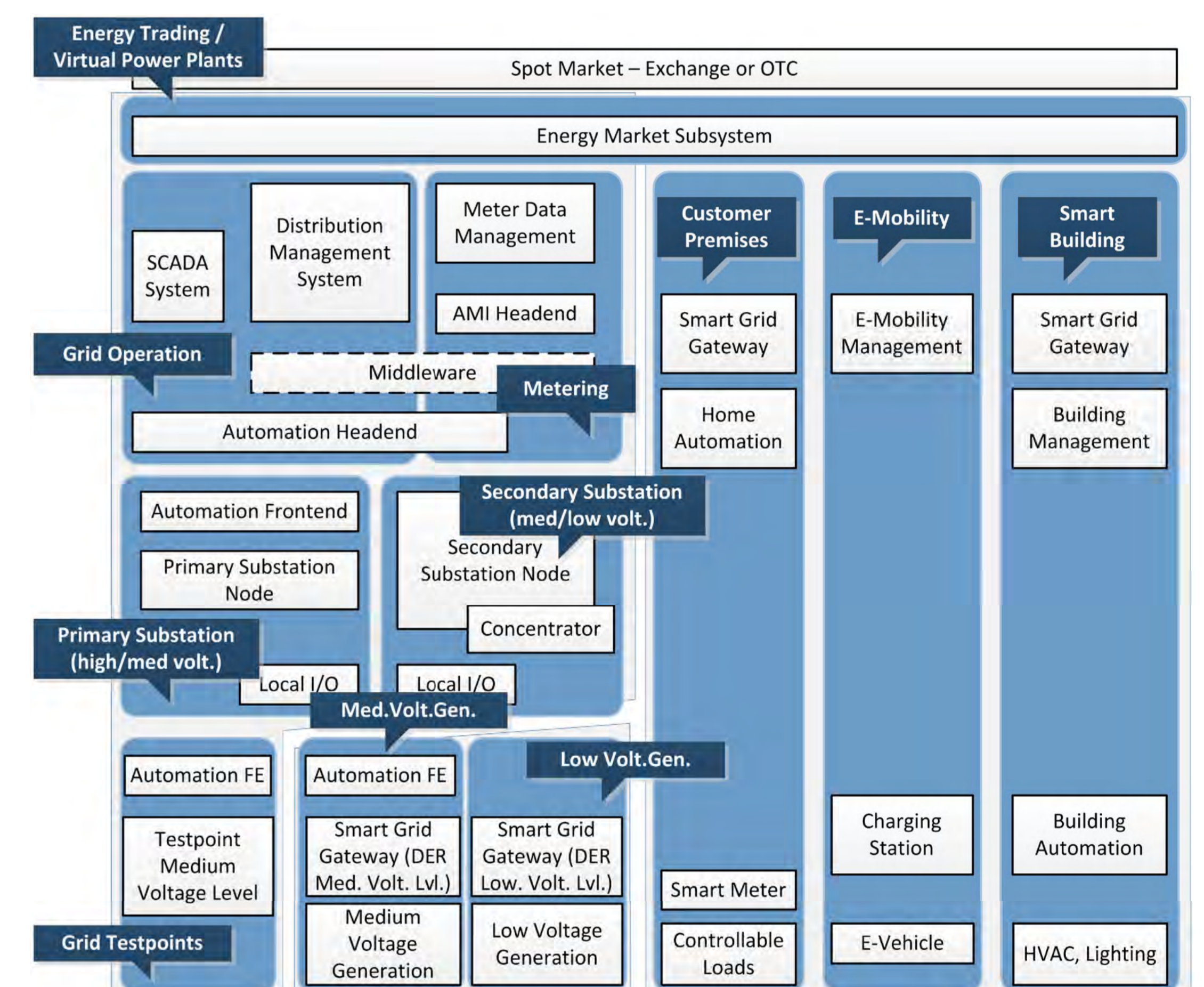
Fig. 2: Clusters of architecture components for risk assessment
