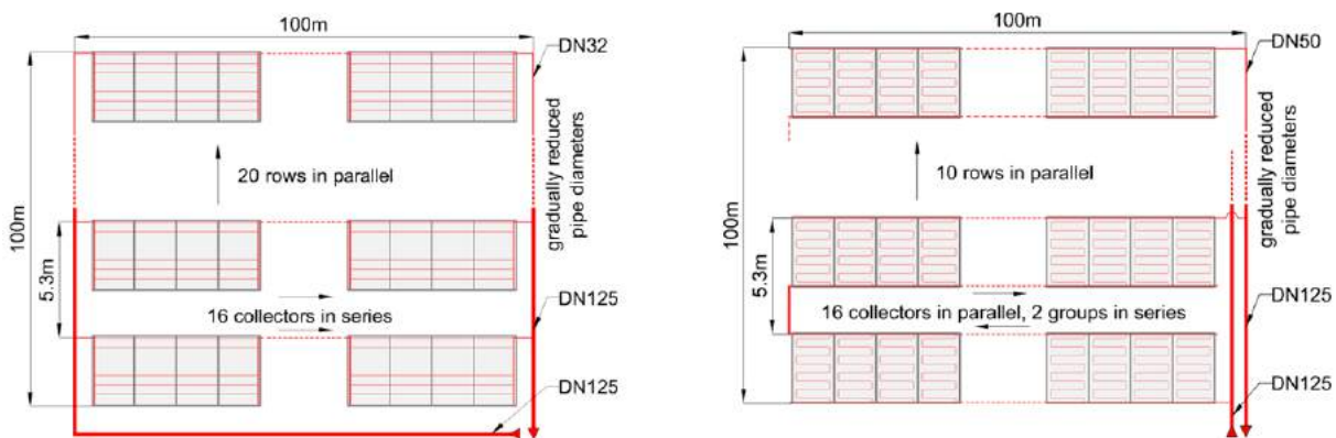
Figure 15: Hydraulic layout of the two reference collector arrays with a gross collector area of 4,800 m² each. The collector array on the left uses harp collectors, the one on the right meander collectors (Philip Ohnewein, 2013).
