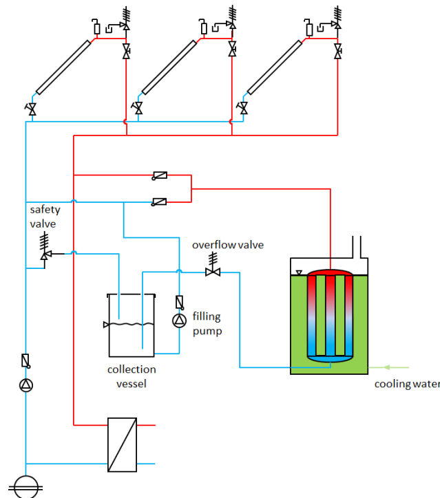
Figure 23: Example hydraulics diagram of a stagnation cooler in solar thermal plant
