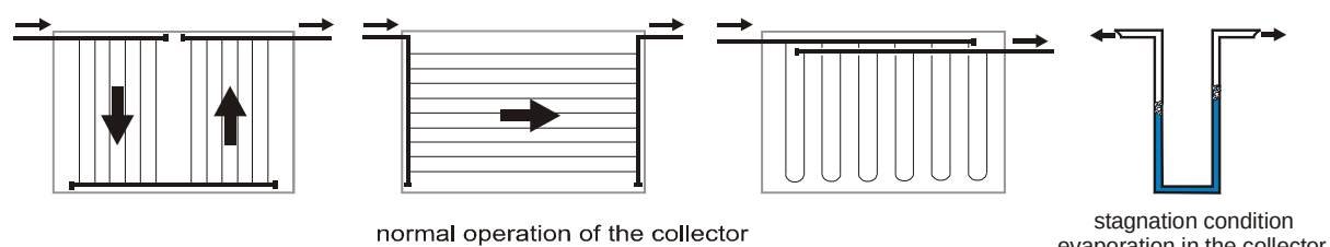
Figure 17: Schematic presentation of different circuitries in collectors with poor emptying behaviour. (Hausner & Fink, 2000)
