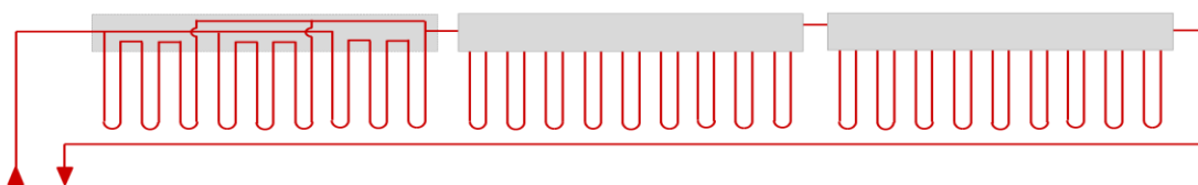
Figure 10: Example collector row hydraulic with direct flow through the evacuated pipes.
