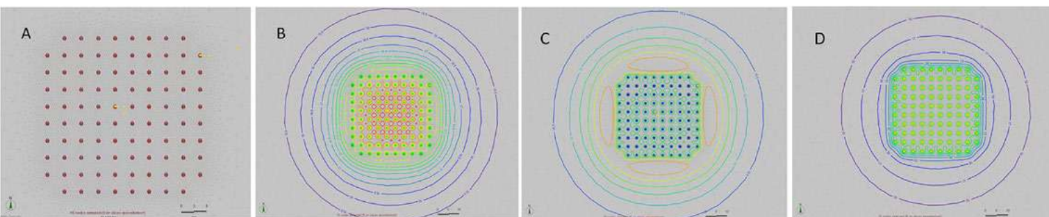
Section through the BHE field model. A: position of the BHE and observation points (yellow). B, C and D: situation in the 10th year of operation on 1 January (midwinter), 15 April (end of heating season) and 31 August (midsummer), image: SANBA project
