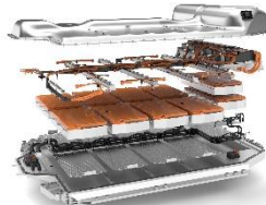
https://www.press.bmwgroup.com/global/photo/detail/P90392467/BMW-Gen5-High-Voltage-Battery-for-BMW-iX3
