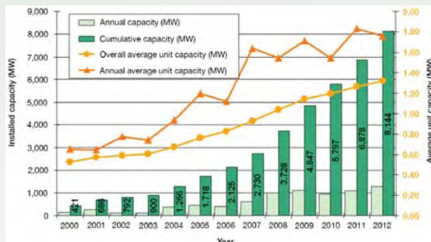
Figure 1. Trend of Italian annual and cumulative wind turbine installed capacity, and newly added and overall average unit capacity
