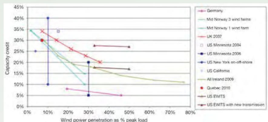
Figure 2. Capacity credit of wind power, results from ten studies, showing reduction of capacity value as penetration level increases. New York on-off-shore shows the range of capacity value for wind, when calculated only for onshore sites (10%) or only offshore sites (40%).
