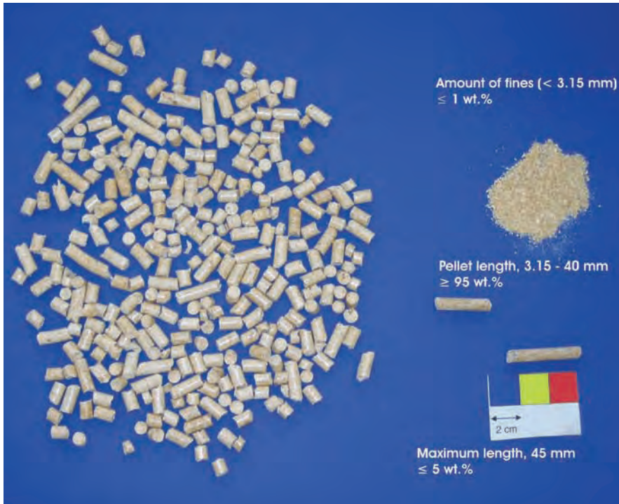
Figure 1: Wood pellet classification according to EN 14961-2. [27]
