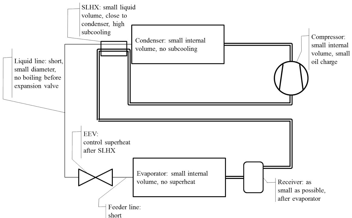
Figure 3. Scheme of a heat pump cycle with its main components and the important design aspects for charge reduction.
