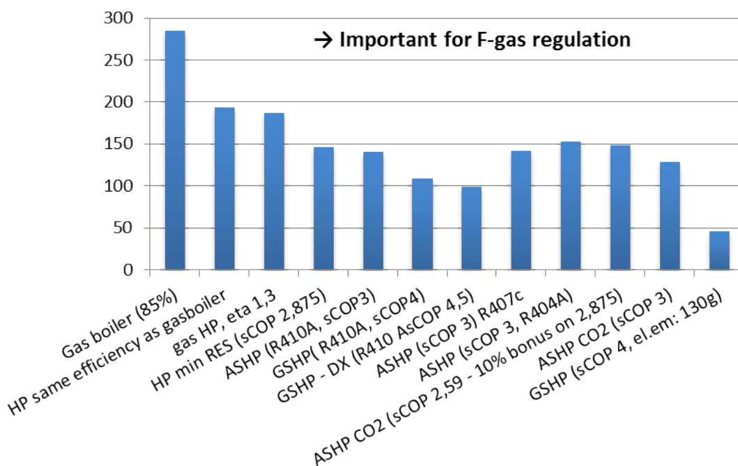
Figure 1. STEWI calculation of different refrigerants (g CO 2 eq/kW th ). [Source: EHPA, European Heat Pump Market and Statistics Report 2013]
