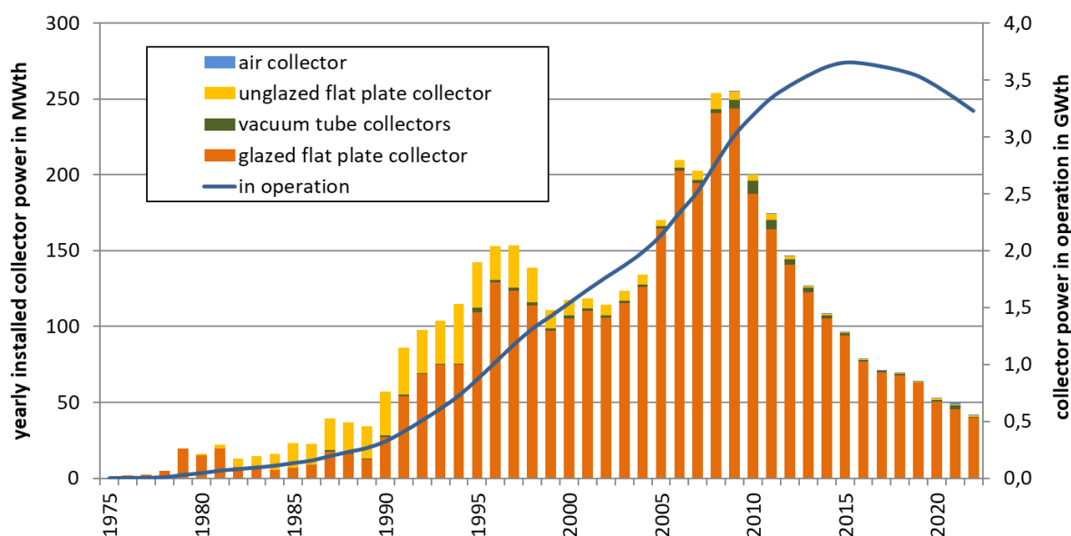
Figure 15 – Market development of solar thermal collectors in Austria until 2022
