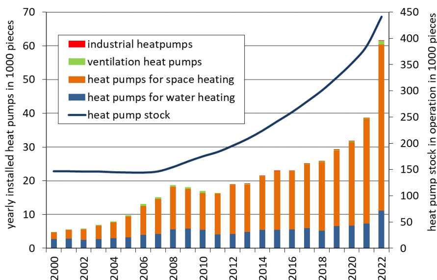
Figure 17 – Market development of heat pumps in Austria until 2022
