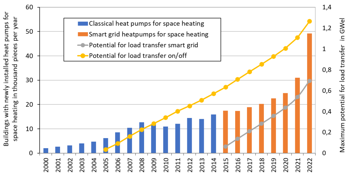
Figure 18 – Development of the grid-beneficial load shift potential with classic and Smart Grid heat pumps in pieces and the resulting load shift potential in GW el . Source: ENFOS (2023)
