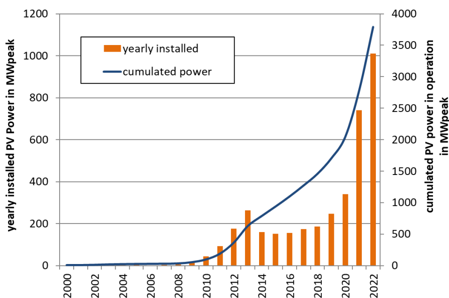
Figure 13 – Market development of photovoltaic systems in Austria until 2022
