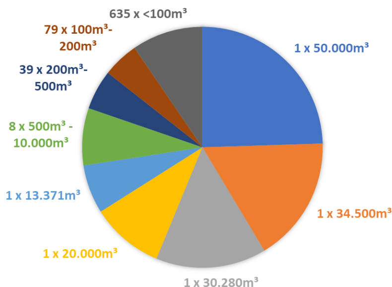
Figure 16 – Distribution of the total volume of tank water storage per surveyed heating network. Data basis: 766 heating networks Source: AEE INTEC (2023)
